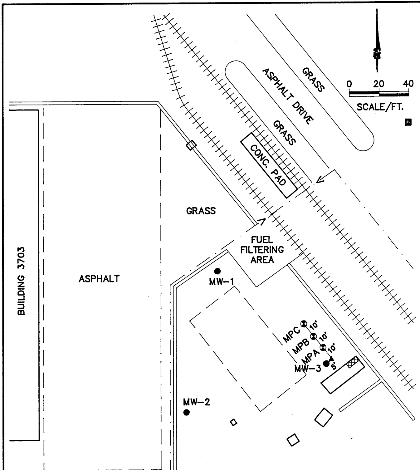
FIGURE 3.1 PROPOSED VENT WELL/ VAPOR MONITORING POINT LOCATIONS POL STORAGE AREA C
