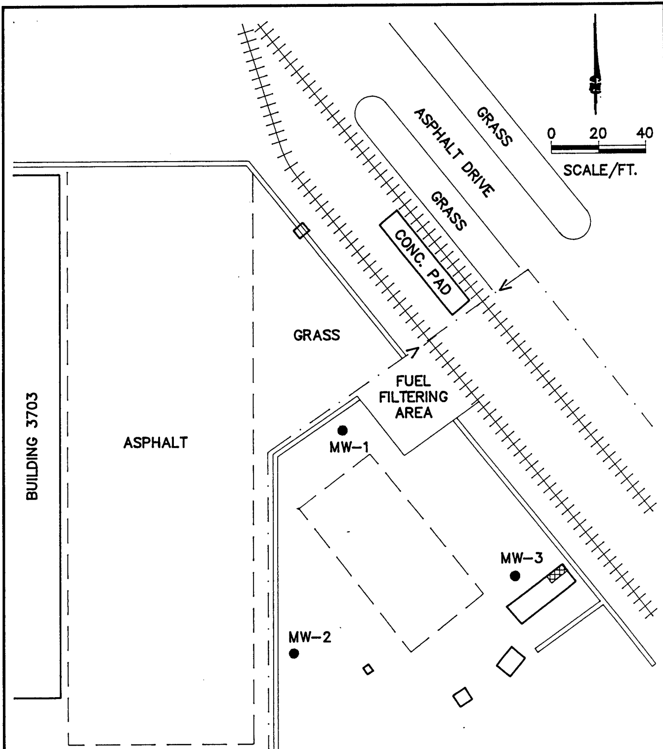
FIGURE 2.2 SITE LAYOUT POL STORAGE AREA C TINKER AFB, OKLAHOMA ENGINEERING-SCIENCE, INC. Denver, Colorado
