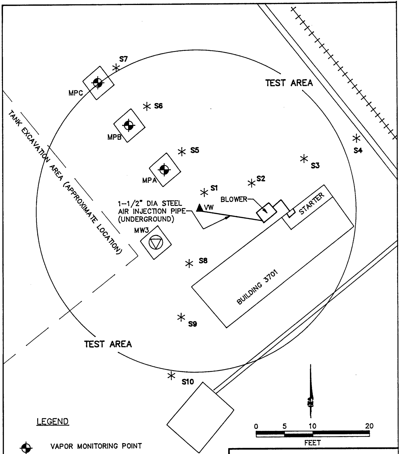
FIGURE 1.1 AS-BUILT VENT WELL, MONITORING POINT, AND BLOWER LOCATIONS POL STORAGE AREA C
