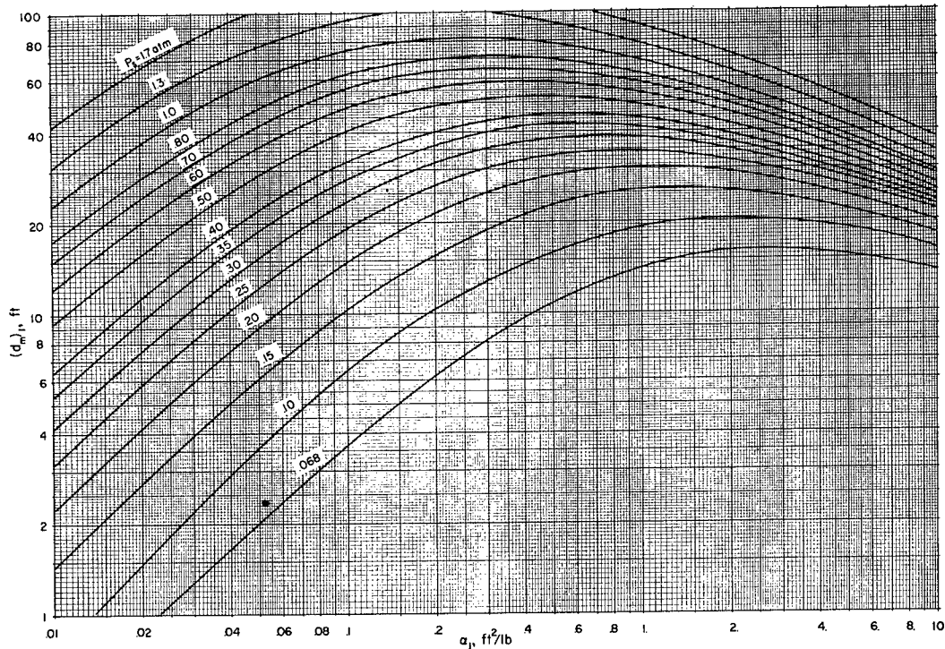
Figure 31 - Predicted displacement at maximum velocity as a function of acceleration coefficient ( a ) and shock overpressure computed for W = 20 kt, \rho_0 = 14.7 psi, and c_0 = 1117 ft/sec. For other conditions use:
