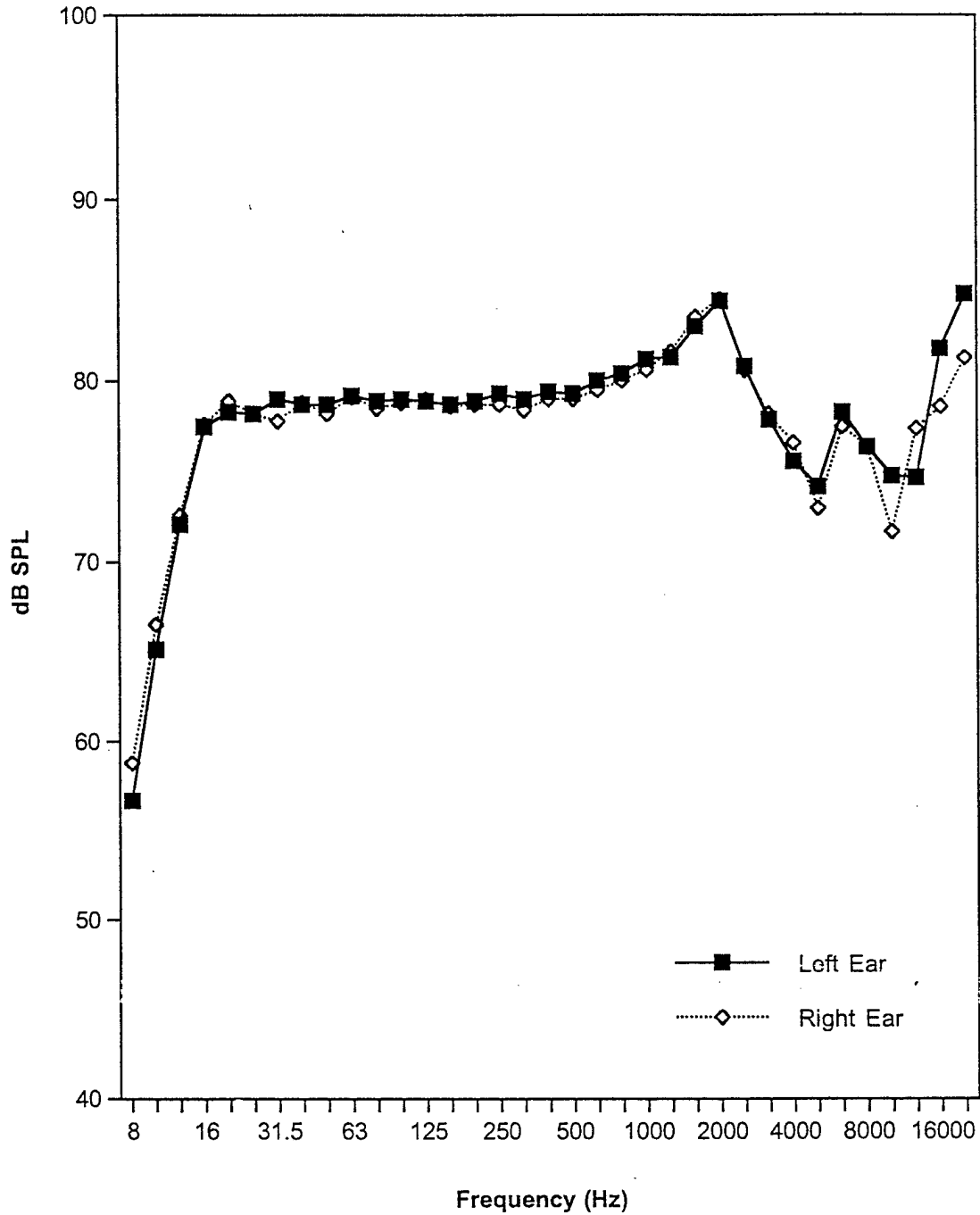
Figure 3: STAX headset frequency response. Differences between left and right earcup output levels against a flat-plate coupler for a STAX (SR-λ) headset, showing negligible divergence. Measurements were made using a pink noise signal source set to produce a nominal level of 85 dB(A) at the coupler.
