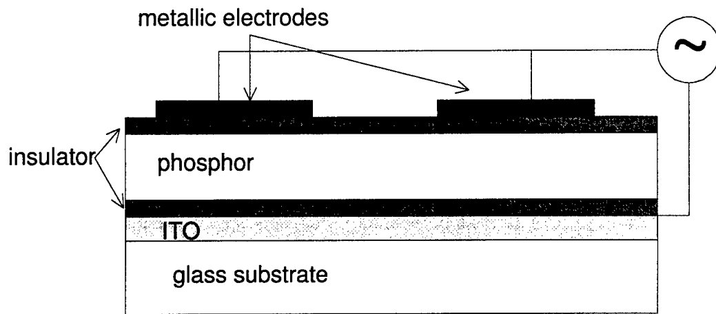
Figure 1.17: A typical electro-luminescent (EL) display cross-section showing the film arrangement needed for a display device, although layers for specific designs may differ.
