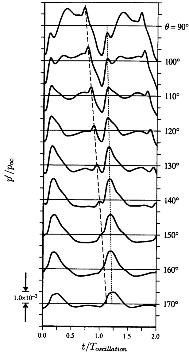
Figure 3.17: Acoustic fluctuation trace at various observation angles \theta , r/\lambda = 1.0 for Case B1. - - - Peak of primary acoustic wave, produced by oblique compression wave - vortex interaction. — — Peak of secondary acoustic wave, produced by traveling compression wave - vortex interaction. Amplitude of primary wave is determined from change in height of sharp compression immediately preceding primary wave peak.
