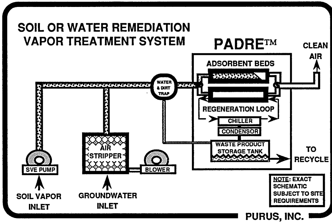
Figure 1. PADRE™ Schematic
