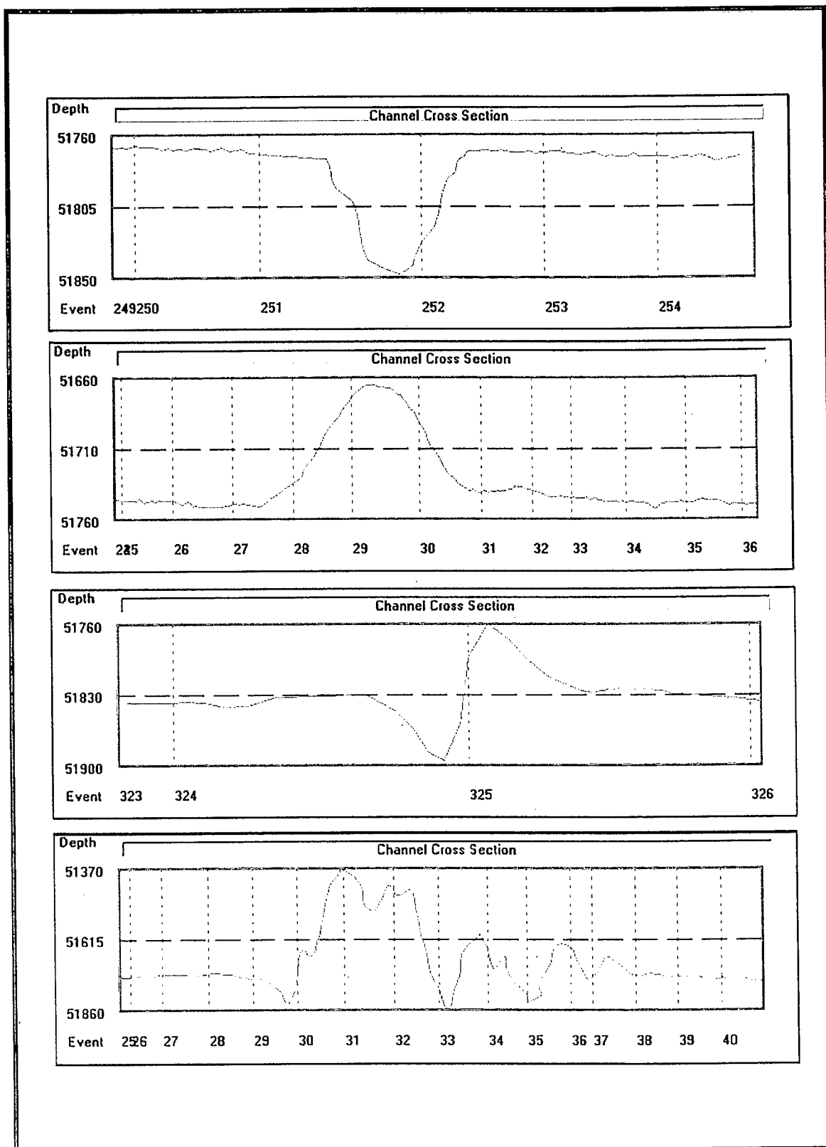
Figure 5. Hypack "Edit" screen images illustrating magnetic anomalies with positive monopolar, negative monopolar, dipolar, and multicomponent signatures. The positive and negative signatures appear inverted, because Hypack records the magnetic readings as "depths"; therefore, "higher" positive readings appear to trend downward rather than upward.
