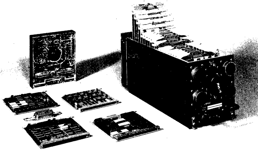
Figure 5 Signal Acquisition and Conditioning Terminal
