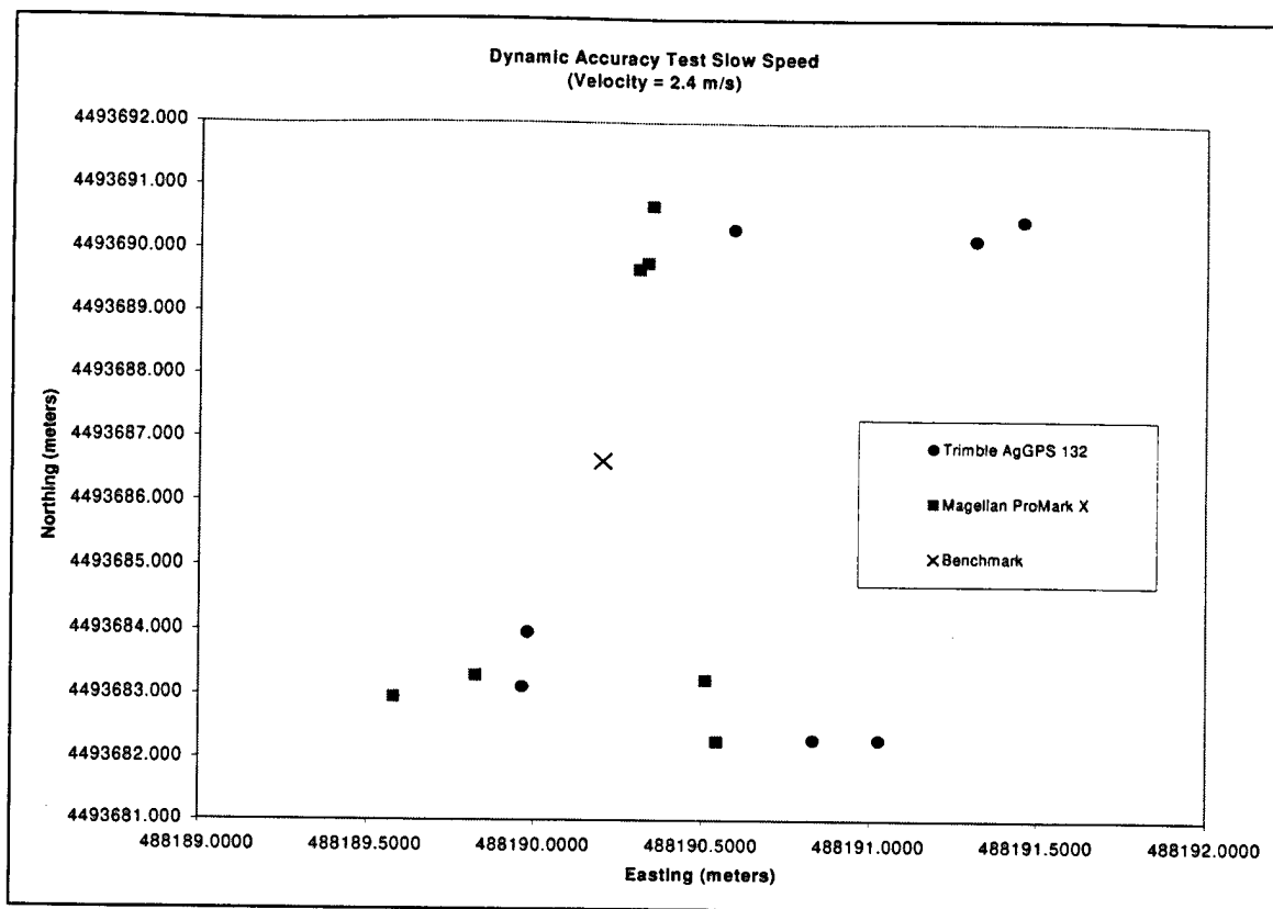
Figure 2. The GPS recorded position at the time the vehicle crossed the benchmark is plotted with the benchmark for comparison.
