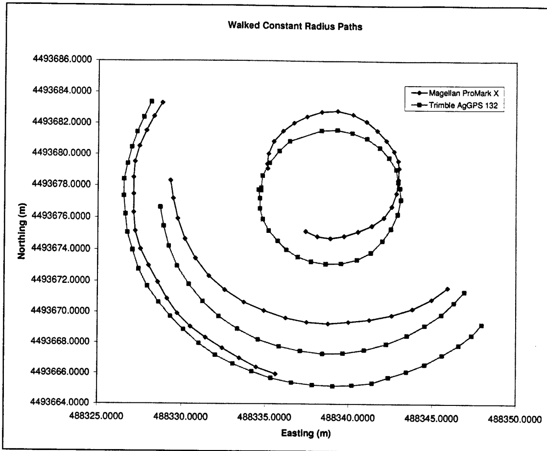
Figure 5. The recorded GPS positions for the calculated turning radius evaluation of paths walked on the level surface.
