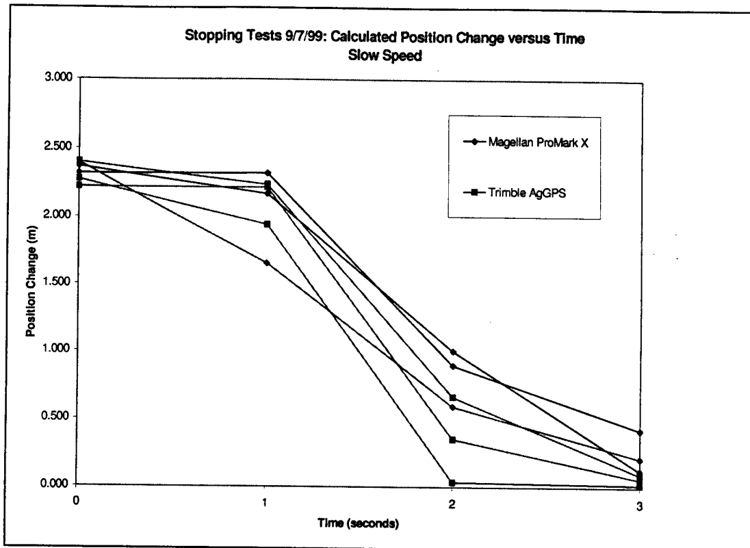
Figure 3. The GPS recorded position change (velocity) for up to 3 seconds after the vehicle had stopped.
