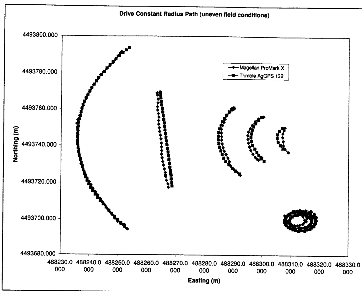
Figure 6. The recorded GPS positions for the calculated turning radius evaluation of paths driven on uneven field conditions.
