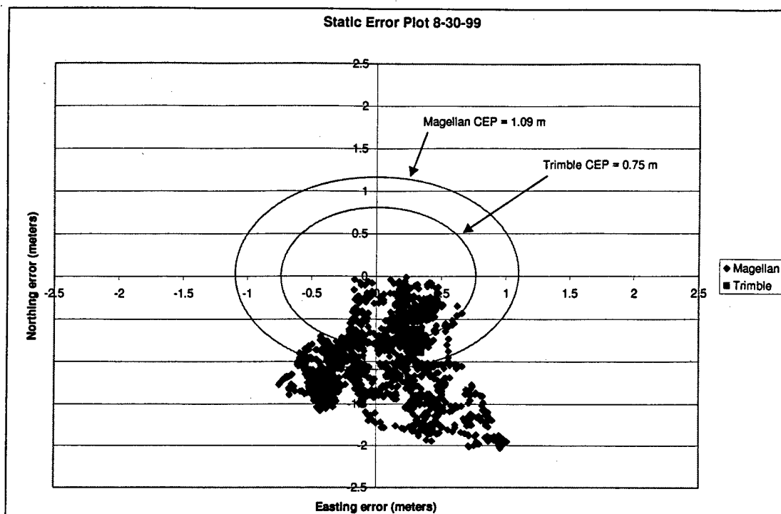
Figure 1. Plot of the difference in position from the GPS position data, recorded on 30 August 1999, to the position of the benchmark.
