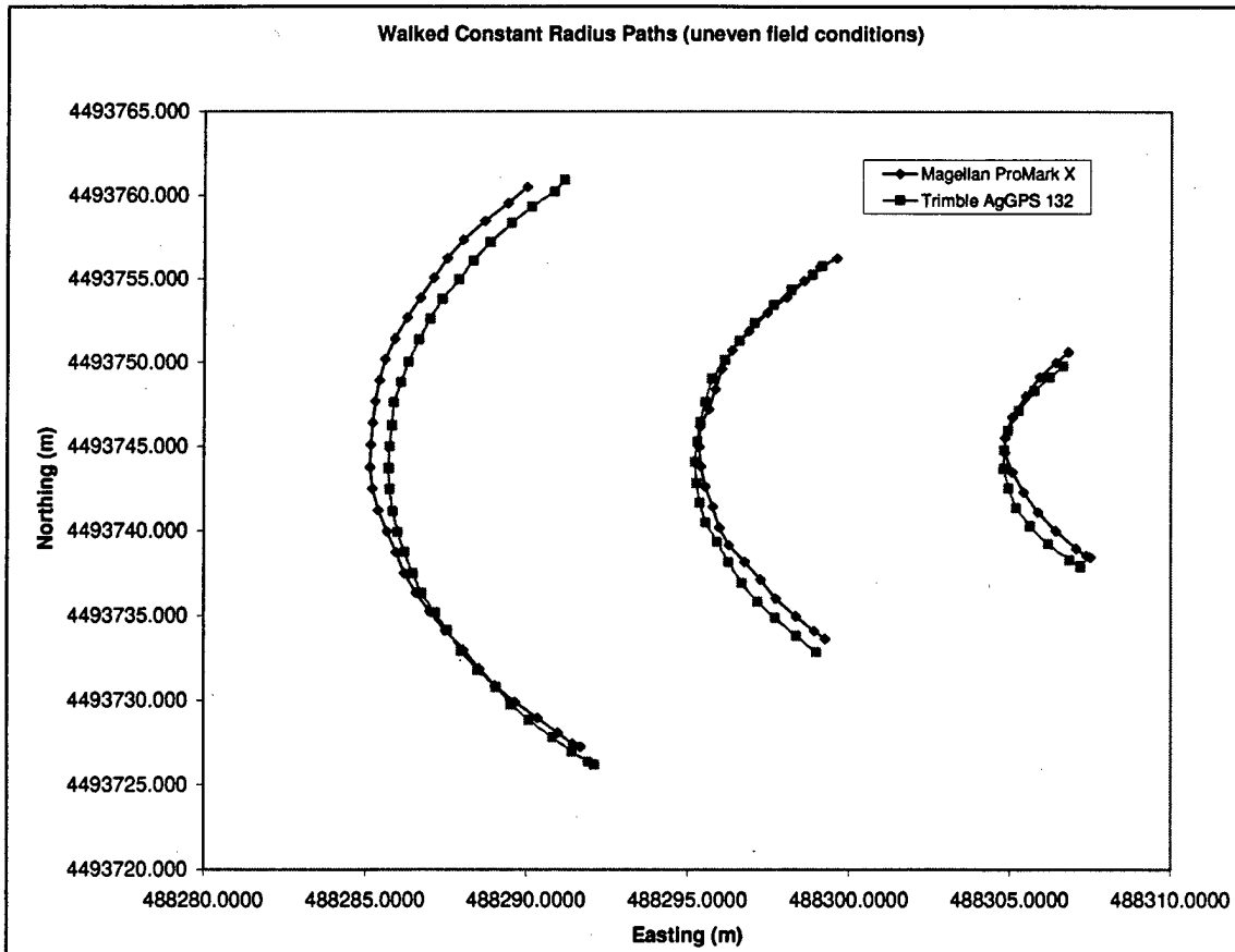
Figure 7. The recorded GPS positions for the calculated turning radius evaluation of paths walked on uneven field conditions.
