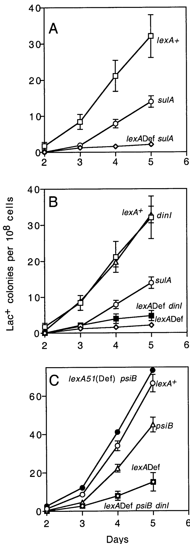
Fig. 3. LexA-repressed inhibitor(s) of Lac + adaptive mutation. (A) Complete de-repression of the LexA regulon inhibits mutation. The lexA defective strain carries lexA51 (Def) suI A211 (◇), lexA + (□), and suI A211 (○). The suI A mutation, required for viability of lexA51 (Def) strains, also depresses mutation modestly (discussed in text). (B) The LexA-controlled inhibitor of adaptive mutation is not DinI. Both lexA51 (Def) strains also carry suI A211. □, dinI + lexA + ; △, dinI ::kan lexA + ; ○, suI A211; ■, lexA51 (Def) suI A211 dinI ::kan; ◇, lexA51 (Def) suI A211. (C) PsiB inhibits adaptive mutation in LexA de-repressed cells. All strains shown carry suI A211. Additional alleles carried are as follows: ○, lexA + ; ●, lexA51 (Def) psiB ::cat; △, psiB ::cat; ◇, lexA51 (Def); ■, lexA51 (Def) psiB ::cat dinI ::kan. Results are discussed in the text.
