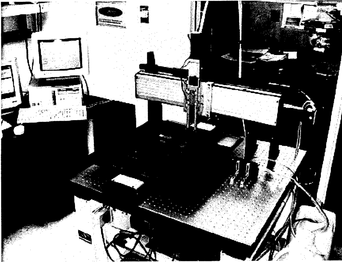
Figure 1: This DNA micro-arrayer built in our laboratory allows to print duplicate arrays on up to 91 slides. When in operation, the instrument is enclosed to maintain a mostly dustfree environment with controlled humidity.
