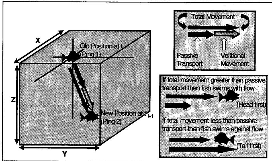
Figure 8. Hydraulic conditions interpolated to the position of the fish can be used to transport the fish through the CFD grid as though it were a neutrally buoyant, passive particle. The predicted location of the fish under passive transport can be subtracted from the known position of the fish at the next ping. The difference between the two distances represents the direction and extent of volitional swimming and the random velocity component by the fish.
