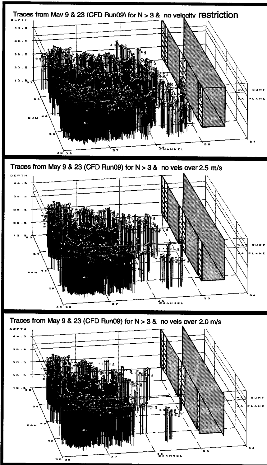
Figure 3. Multi-beam hydroacoustics data with SBC represented as shaded channel (dam to right). Subplot A contains all hydroacoustics data, Subplot B contains traces in which all targets had a calculated velocity less than 2.5 \text{ m s}^{-1} ( 8.2 \text{ ft s}^{-1} ), and Subplot C contains traces in which all targets had a calculated velocity less than 2.0 \text{ m s}^{-1} ( 6.6 \text{ ft s}^{-1} ). Target velocities are not corrected for passive transport.
