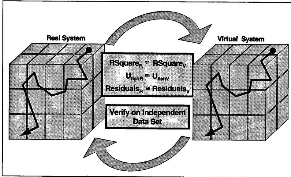
Figure 12. Future methods for calibrating behavior models. In a coupled Eulerian-Lagrangian framework, the adequacy of the simulation can be determined by how well the results of statistical analysis of the virtual system matches the statistical analysis of the real system in terms of R-Square, variables and their weights, and behavior of the residuals.
