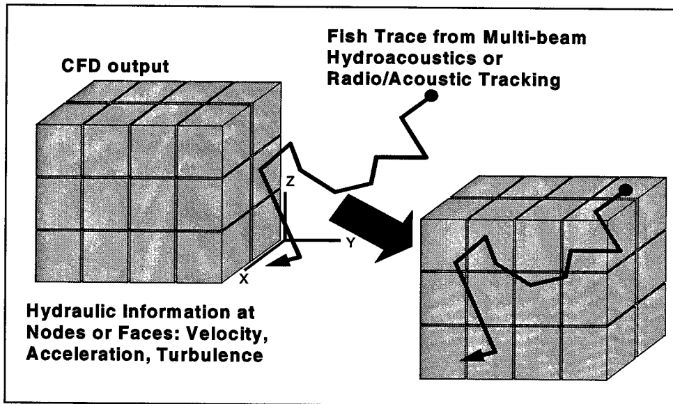
Figure 4. Conceptualization of how 3-dimensional hydroacoustics data and idealized output grid of CFD modeling are placed into a common coordinate system. Once combined, hydraulic information nearest each successive location estimate can be identified and used to develop statistical relationships between swim path selection and hydraulic conditions.
