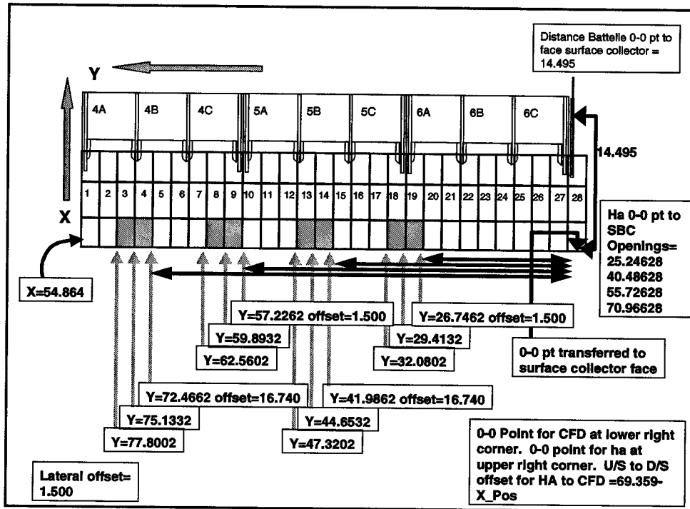
Figure 2. Plan view of Lower Granite Dam surface collector schematic (all distances in meters from the 0,0 point). Using the project design plans as an intermediate step, openings to the surface collector were used as common reference points for the two data sets. Hydroacoustics data (HA) set spatial referencing system (black lines) was adjusted to match the CFD grid (gray lines).
