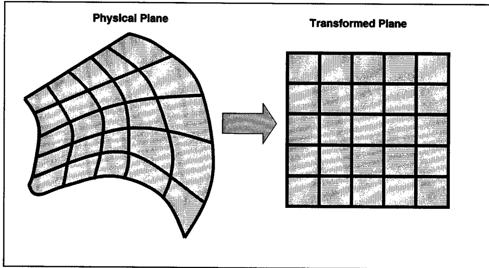
Figure 13. Transforming physical space to contravariant space allows all computations and georeferencing to be performed in unit square space for planes and unit cubed space for volumes. Use of contravariant space for biological data collection will considerably ease data merging.
