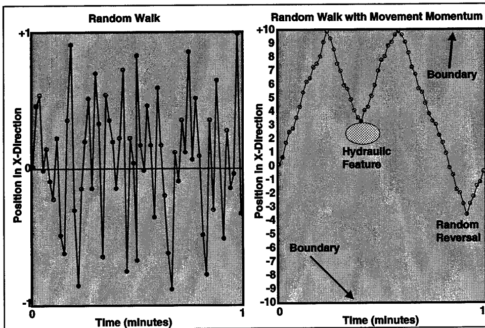
Figure 7. Comparison of traces expected from modeling movement as a random walk (left subplot) versus modeling movement as random process in which the distance traveled is random but direction of movement is conserved between one steps (right subplot). Direction of movement will change when either a repelling hydraulic feature is encountered or when a random reversal in movement occurs.
