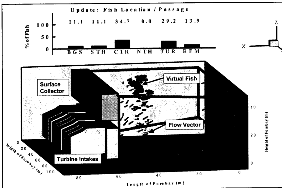
Figure 15. Example of the decision-support shell that can be used to evaluate different fish passage designs or operational plans. Legend: BGS = surface collector opening nearest the behavioral guidance system, STH = south opening to the SBC, CTR = center opening of the SBC, NTH = north opening to the SBC, TUR = turbines, REM = remaining fish in the simulation.
