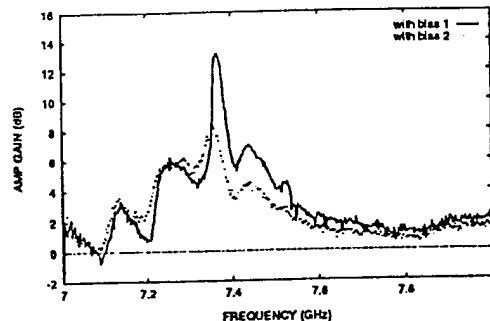
Figure 8: Amplifier gain for configuration 3.
