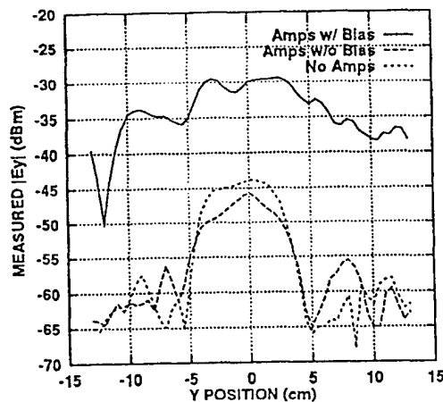
Figure 9: |E_v| pattern on the top surface of slab. This pattern is measured at 7.38GHz with P_{in} = 10 dBm
