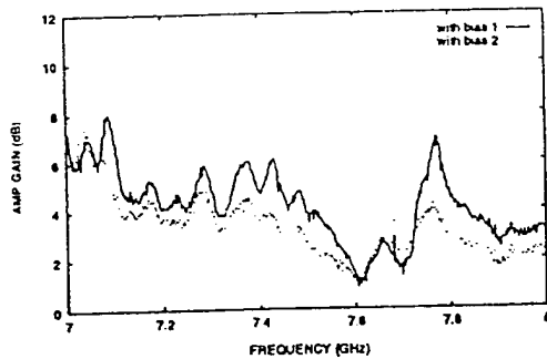
Figure 6: Amplifier gain for configuration 2.
