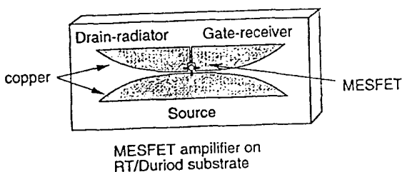
Figure 4: MESFET Vivaldi amplifier
