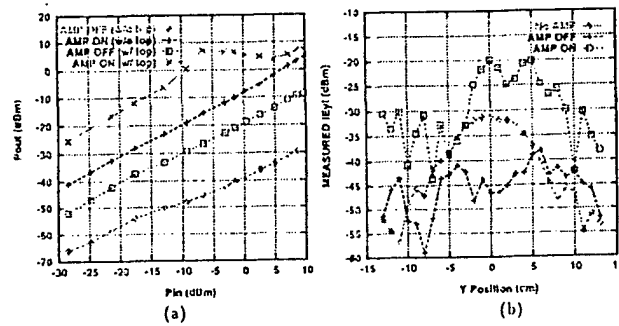
Figure 4: (a) P_{in} vs P_{out} at 8.828 GHz. (b) Measured |E_y| patterns for the system with a 5x4 array working at 8.828 GHz.
