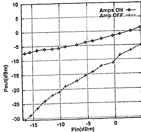
Figure 7: P_{out} vs P_{in} as amplifiers with/without bias
