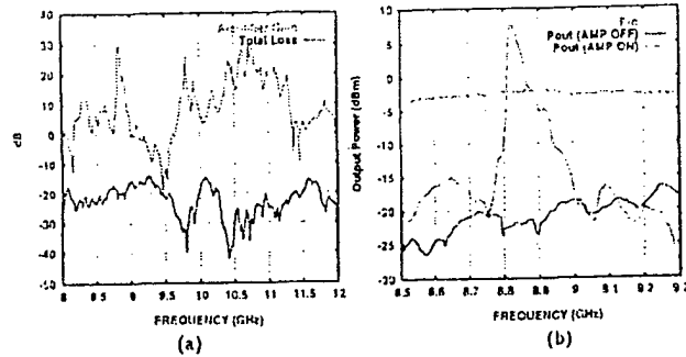
Figure 3: (a) Amplifier gain and total loss for the system with a 5x4 array. (b) P_{out} vs frequency for the system with a 5x4 array.
