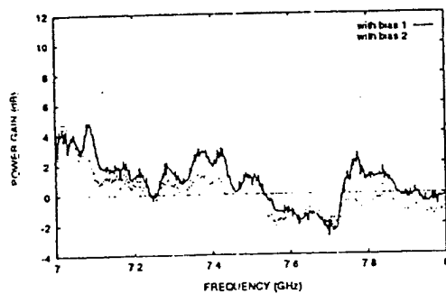
Figure 7: Power gain for configuration 2.
