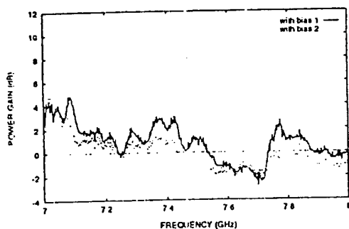
Figure 7: Power gain for configuration 2.
