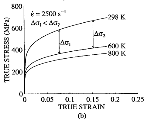
Fig. 1. Stress-strain relations of tantalum predicted by the Johnson-Cook model using the material parameters given by Chen and Gray (1995) (a) different strain rates 10^{-3} , 10^{-1} , and 2500 \text{ s}^{-1} , same temperature (298K); (b) different temperatures (298, 600, and 800K), same strain rate ( 2500 \text{ s}^{-1} ).
