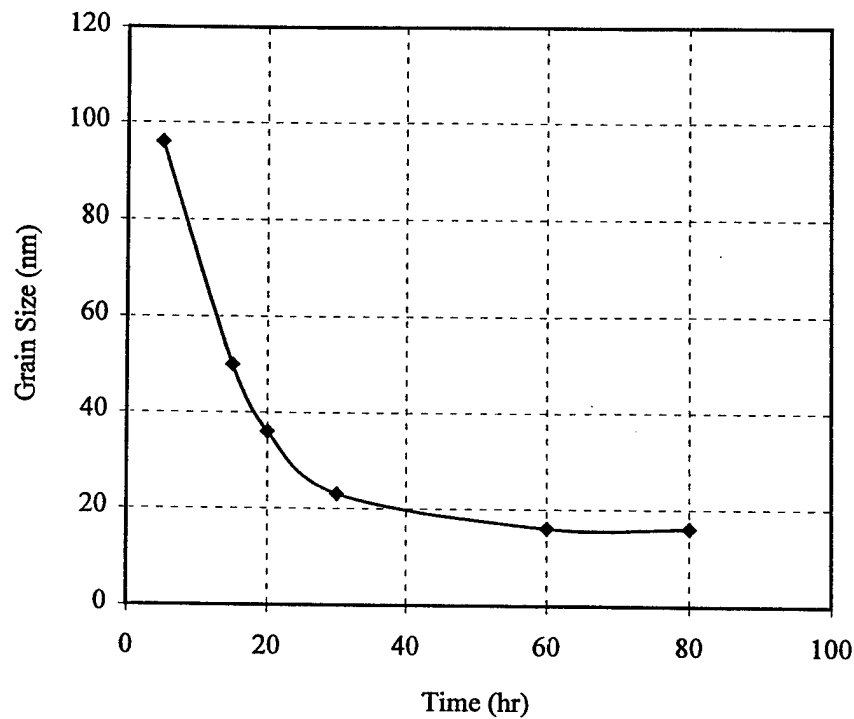
Fig. 2. Grain size of iron powder versus milling time.
