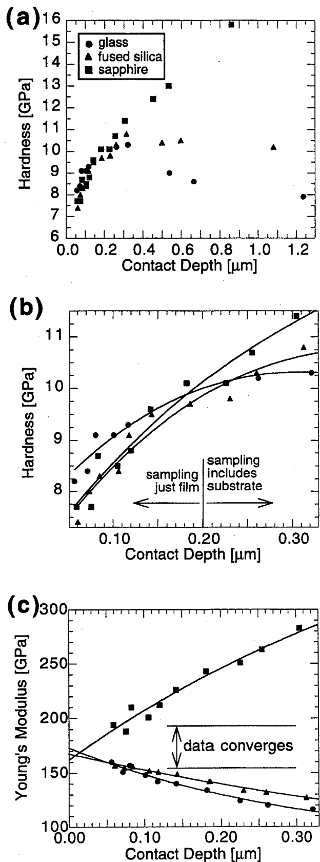
Fig. 6. Summary of results from nanoindentation experiments performed on identical samples with various substrates. (a) Hardness for each indentation is plotted vs. contact depth of indenter tip. Effects from substrate dominate results for large contact depths where hardness curves diverge. (b) Magnified convergence region of Fig. 6a showing for smaller contact depths hardness values obtained by sampling just film. Hardness decreases from ~10 GPa when sampling nearly the entire multilayer, to ~8 GPa when sampling just the top-most layers of laminate. (c) Young's modulus for each indentation is plotted vs. contact depth of indenter tip. Values obtained give upper and lower limit of 195 and 156 GPa for Young's modulus of films.
