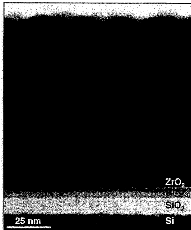
Fig. 3. Bright-field transmission electron micrograph illustrating overall nanolaminate structure of film B. Zirconia and alumina layers are each about 5 nm thick and silicon substrate is shown at bottom of image. Micrograph shows laminate structure of film loses definition away from substrate.
