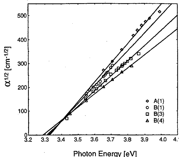
FIG. 6. \alpha^{1/2} vs photon energy for film states A_1 , B_1 , B_3 , and B_4 that are predominantly anatase+amorphous. The intersection of these lines defines E_g=3.41 eV for a nonrutile virtual crystal. The intersection of these lines with the abscissa defines E_x=3.33 eV for A_1 , 3.32 eV for B_1 , 3.31 eV for B_3 , and 3.29 eV for B_4 (see Table V).
