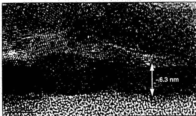
Fig. 10. HRTEM of a 110-nm thick zirconia layer (film E) showing example of pocket commonly observed in films D and E. Measurements of the pocket's distance from the substrate, on this and similar structures, give an average distance of 6.3 nm from the substrate. This value coincides with value of 6.2 nm for the critical size for spontaneous tetragonal to monoclinic transformation predicted by end-point thermodynamics calculations.
