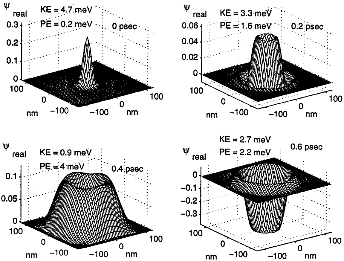
Figure 2. Time-domain evolution of the testing function initiated at the center of the two-dimensional harmonic oscillator potential. The original testing function is a Gaussian pulse of 15 nm. Note that the total energy of the function remains constant, but there is an exchange between kinetic and potential energy. (Only the real part of the wavefunction is shown.)
