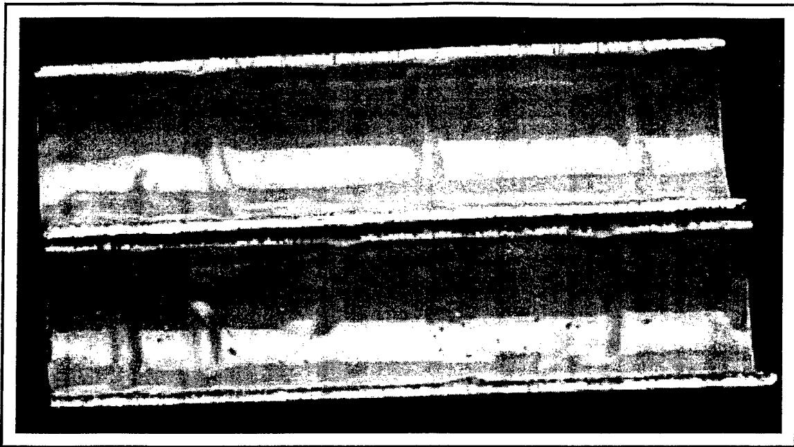
Figure B3. Specimen C14 (in-situ epoxy coating, soft water, 5 fps).
