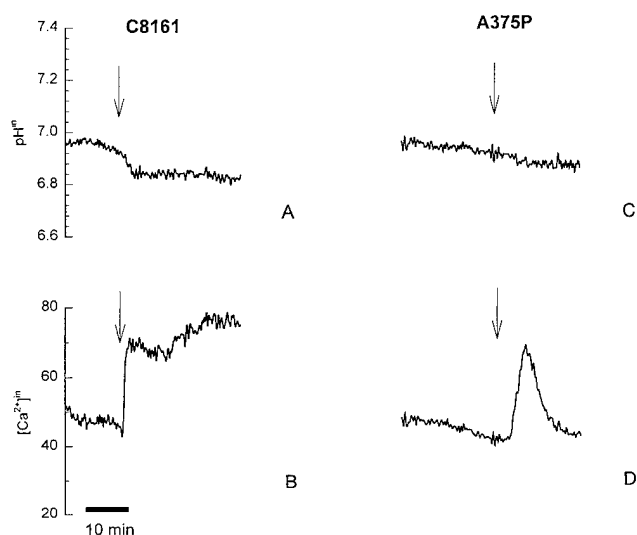
Fig. 3. Effect of the Ca 2+ ionophore, 4Br-A23187, on pH in and [Ca 2+ ] in in highly metastatic C8161 (A,B) and poorly metastatic A375P (C,D) human melanoma cells. Cells were handled as described in Figure 1 and co-loaded with SNARF-1 and Fura-2 to simultaneously measure pH in and [Ca 2+ ] in , respectively. Perfusion begun with HCO 3 - -free CSB, pH ex 7.15. At the time indicated, the perfusate was exchanged for one containing 1 μM 4Br-A23187 in HCO 3 - -free CSB (arrows). Data are representative of eight experiments.
