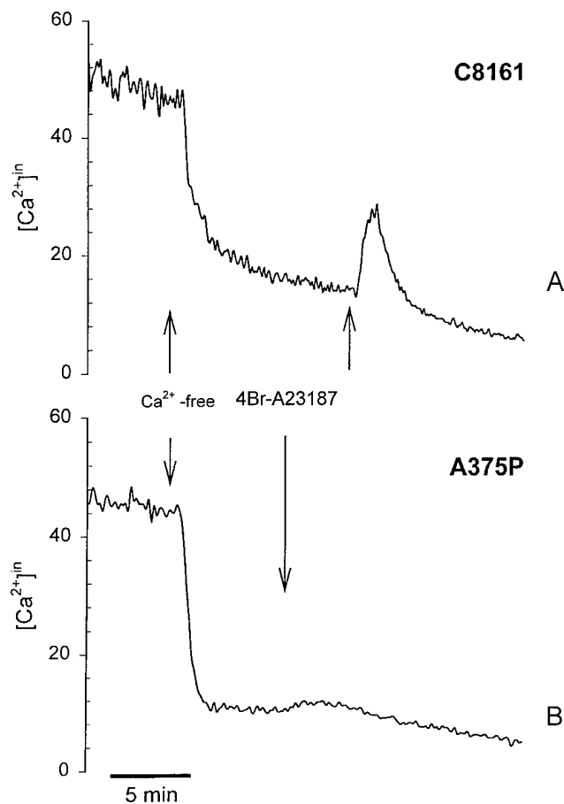
Fig. 5. Effect of [Ca^{2+}]^{\text{ex}} removal and 4Br-A23187 treatment on [Ca^{2+}]^{\text{in}} in highly metastatic (A) C8161 and poorly metastatic (B) A375P human melanoma cells. Cells were handled as described in Figure 3, except that at the time indicated (first arrow), media was exchanged for one lacking Ca^{2+} (supplemented with 1 mM EGTA). At the second arrow, perfusate was exchanged for one containing 1 \mu M 4Br-A23187, in a Ca^{2+} free buffer. Data are representative of nine and eight experiments performed in C8161 and A375P cells, respectively.
