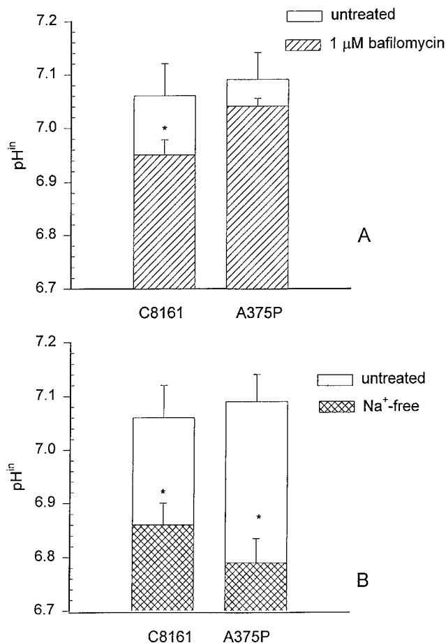
Fig. 6. Effect of bafilomycin, a V-type H^+ -ATPase inhibitor (A), and Na^+ -removal (B), on pH^{\text{in}} in highly metastatic C8161 and poorly metastatic A375P melanoma cells. Cells were grown onto coverslips and loaded with SNARF-1 to measure pH^{\text{in}} , as previously described (Martínez-Zaguilán et al., 1993). Subsequently, cells were transferred to the fluorometer cuvette and perfusate begun with HCO_3^- -free CSB at a pH^{\text{ex}} = 7.15 . Once steady-state pH^{\text{in}} was reached, perfusate was exchanged for one containing 1 \mu M bafilomycin A_1 , a V-type H^+ -ATPase inhibitor (A). Alternatively, perfusate was exchanged for a Na^+ - and HCO_3^- -free CSB at a pH^{\text{ex}} = 7.15 . Na^+ was substituted with N-Methyl glucamine to maintain osmotic equilibrium (B). The newly resting pH after either bafilomycin addition or Na^+ -removal was obtained once equilibrium was established, typically after 5 min. Data represents the mean \pm S.D. of seven experiments for each condition. * P < 0.05 for the following conditions: (a) bafilomycin treated versus untreated C8161 cells; (b) magnitude of the pH^{\text{in}} decrease following Na^+ removal in both A375P and C8161 cells; (c) magnitude of the acidification following Na^+ removal is significantly larger in A375P than in C8161 cells. There were no significant differences in neither steady-state pH^{\text{in}} between C8161 and A375P cells, or following bafilomycin treatment in A375P cells.
