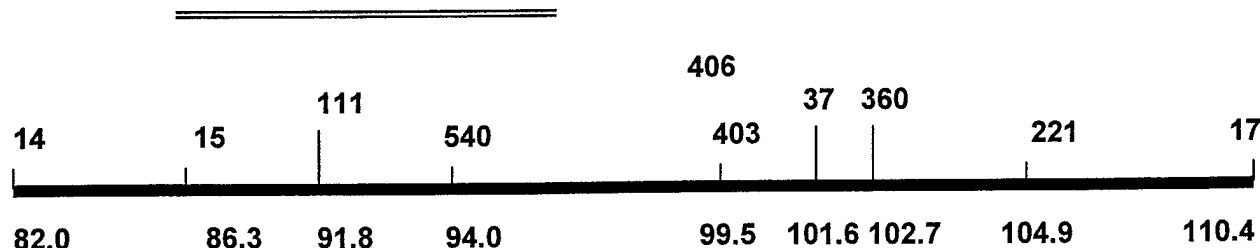
Figure 3. Subcongenic Lines of QTL Region. The double line represent the region covered by each of the subcongenic lines. The solid bar at the bottom represents the original region of the chromosome of CAST within the congenic strain. Numbers above the bar represent the position and names of D1mit microsatellite markers while the number under the bar represent the cM distance on the mouse chromosome 1.
