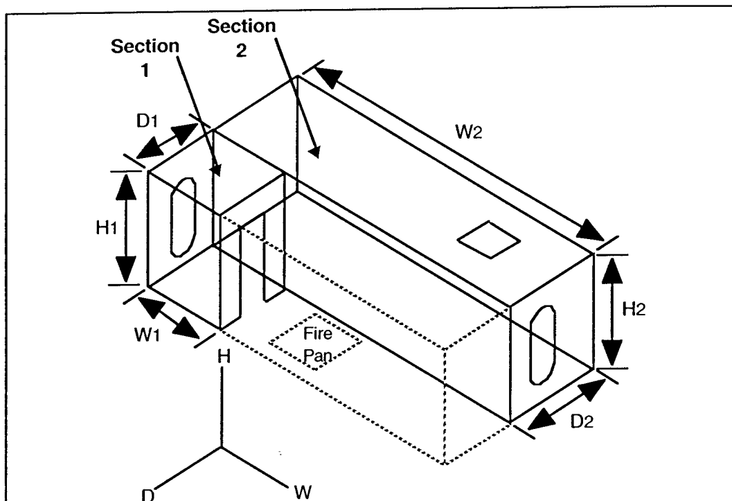
Figure 11. Equivalent Geometry of the Laundry Passageway for the Three-Compartment Model
