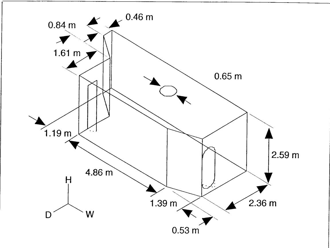
Figure 22. Control Room Dimensions
