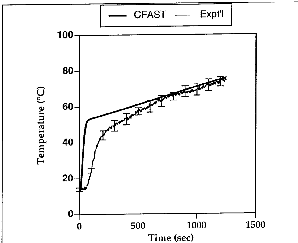
Figure 32. Predicted versus Measured Upper Layer Gas Temperatures for the Navigation Equipment Room
