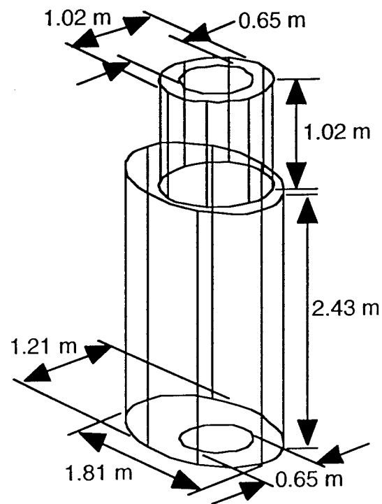
Figure 24. Sail Dimensions
