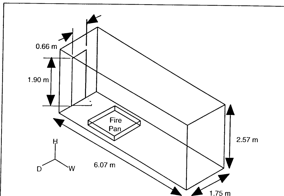
Figure 3. Laundry Room Configuration
