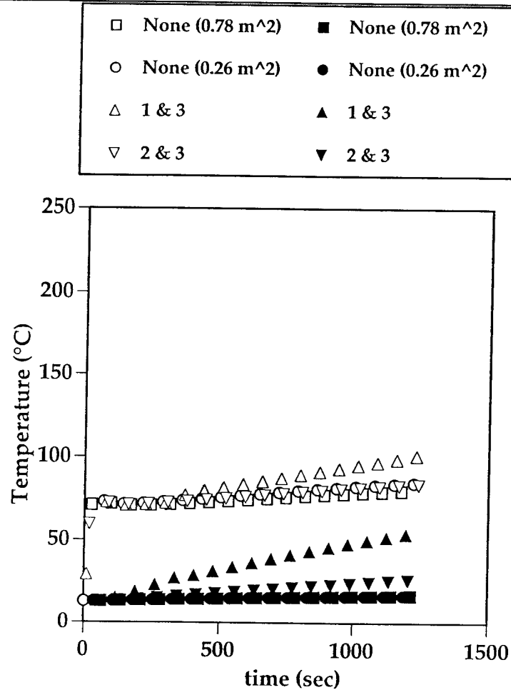
Figure 18. Effects of Vertical Conduction on Wardroom Gas Temperatures
