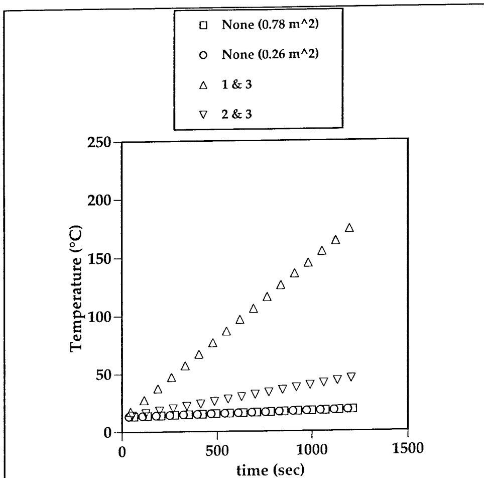
Figure 19. Effects of Vertical Conduction on Wardroom Deck Temperature
