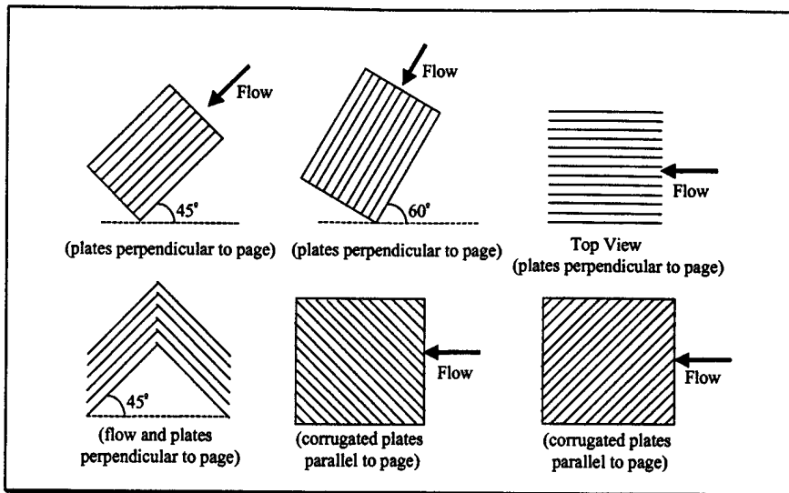
Figure 3. Coalescer configurations.
