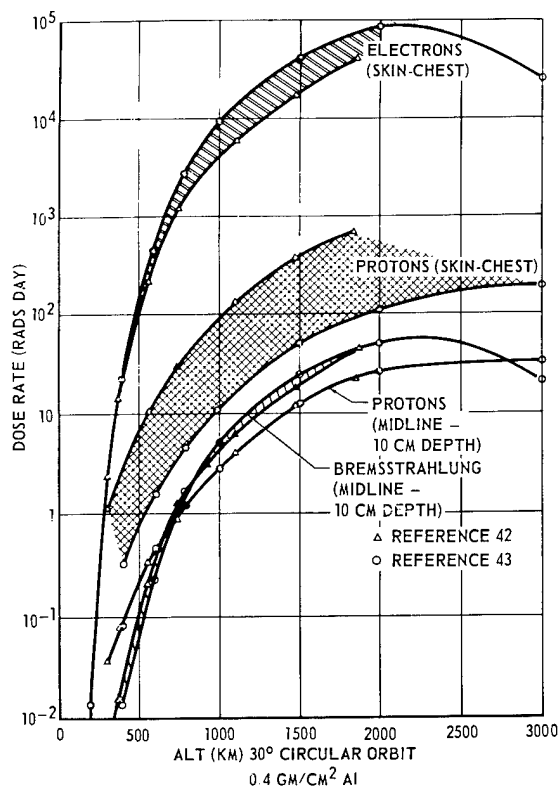
Figure II-5. Dose rate as a function of circular orbital altitude ( 30^\circ inclination, 0.4 \text{ g/cm}^2 Al shielding).
