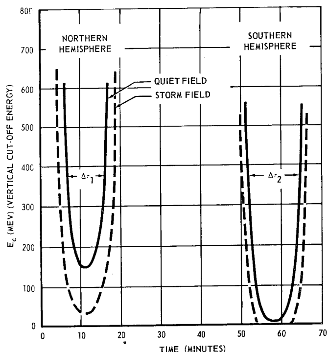
Figure II-11. Variation of magnetic cut-off energy with time for first orbit [ 60^\circ inclination and 200-n.m. ( \sim 400 -km) altitude].
