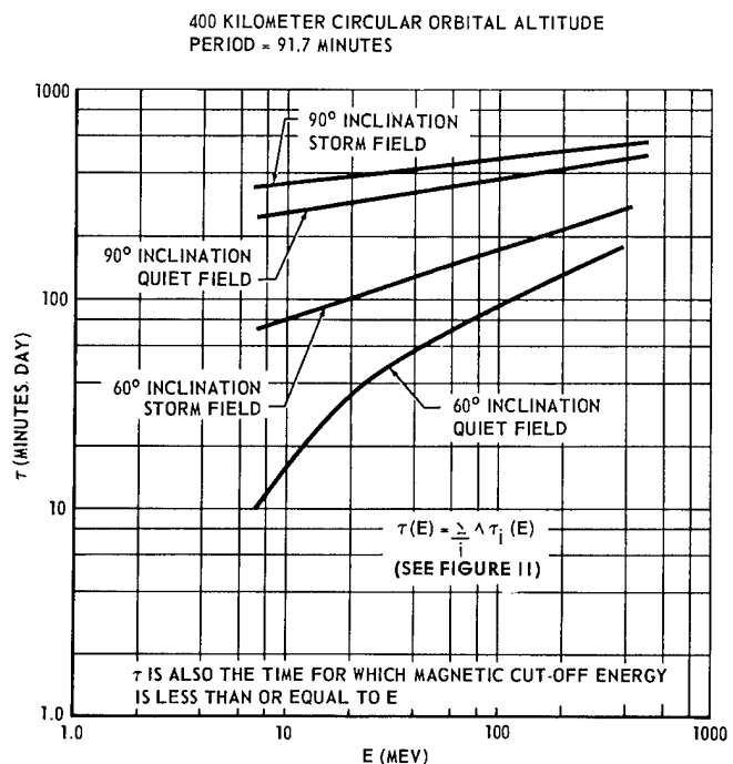
Figure II-10. Time exposed to protons of energy greater or equal to E for 200-n.m. ( \sim 400 -km) circular orbit with 60^\circ and 90^\circ inclinations.
