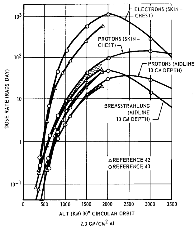
Figure II-6. Dose rate as a function of circular orbital altitude ( 30^\circ inclination, 2 \text{ g/cm}^2 Al shielding).
