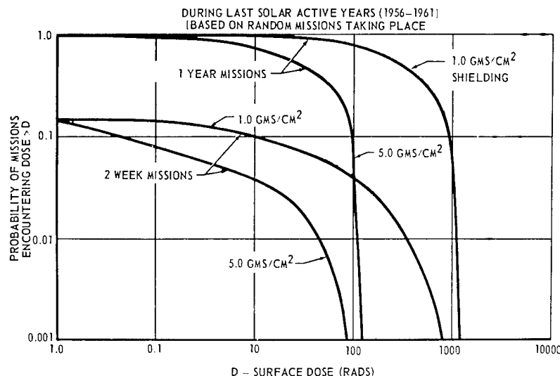
Figure II-9. Probability of missions of 2 weeks and 1 year duration encountering a surface dose greater than D (for shielding thicknesses of 1 and 5 \text{g}/\text{cm}^2 ) during last solar-active years (1956-1961).
