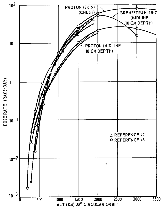
Figure II-7. Dose rate as a function of circular orbital altitude ( 30^\circ inclination, 5 \text{ g/cm}^2 Al shielding).
