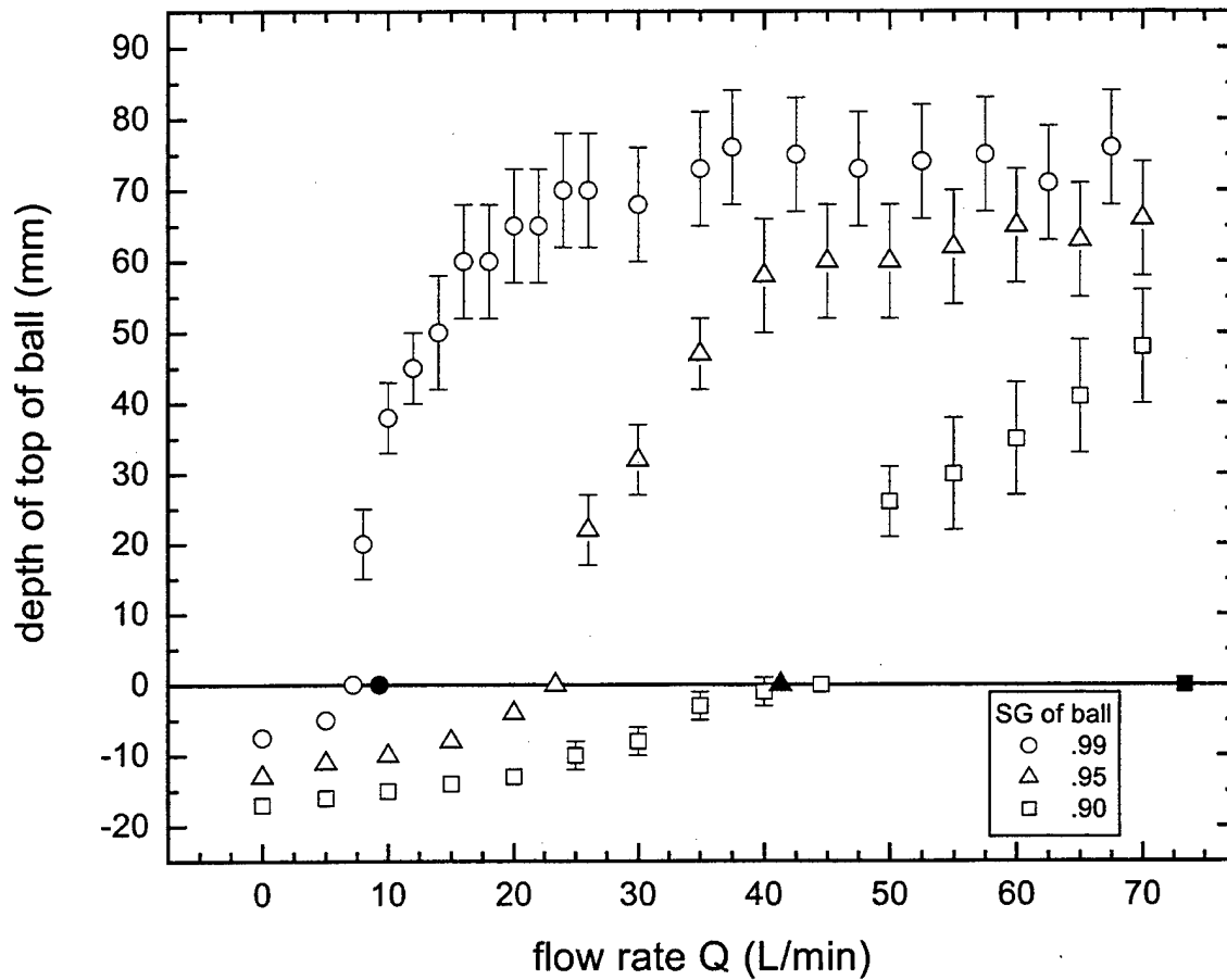
Figure 5.4. Depth of ball vs. flow rate for three selected specific gravities of the density ball. Filled-in (black) symbols indicate the flow rate the ball would have sunk in the closed environment.
