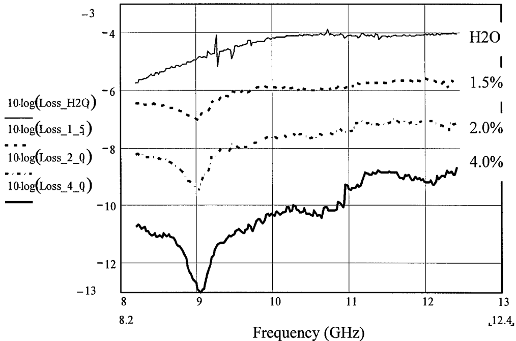
Figure 8. (Same as Figure 1) Power dissipated inside solution filled capillaries, \text{Power}_{\text{absorbed}} = 1 - |S_{11}|^2 - |S_{12}|^2 , in X-band waveguide test set-up. The presence of a resonance region is clear near 9 GHz.
