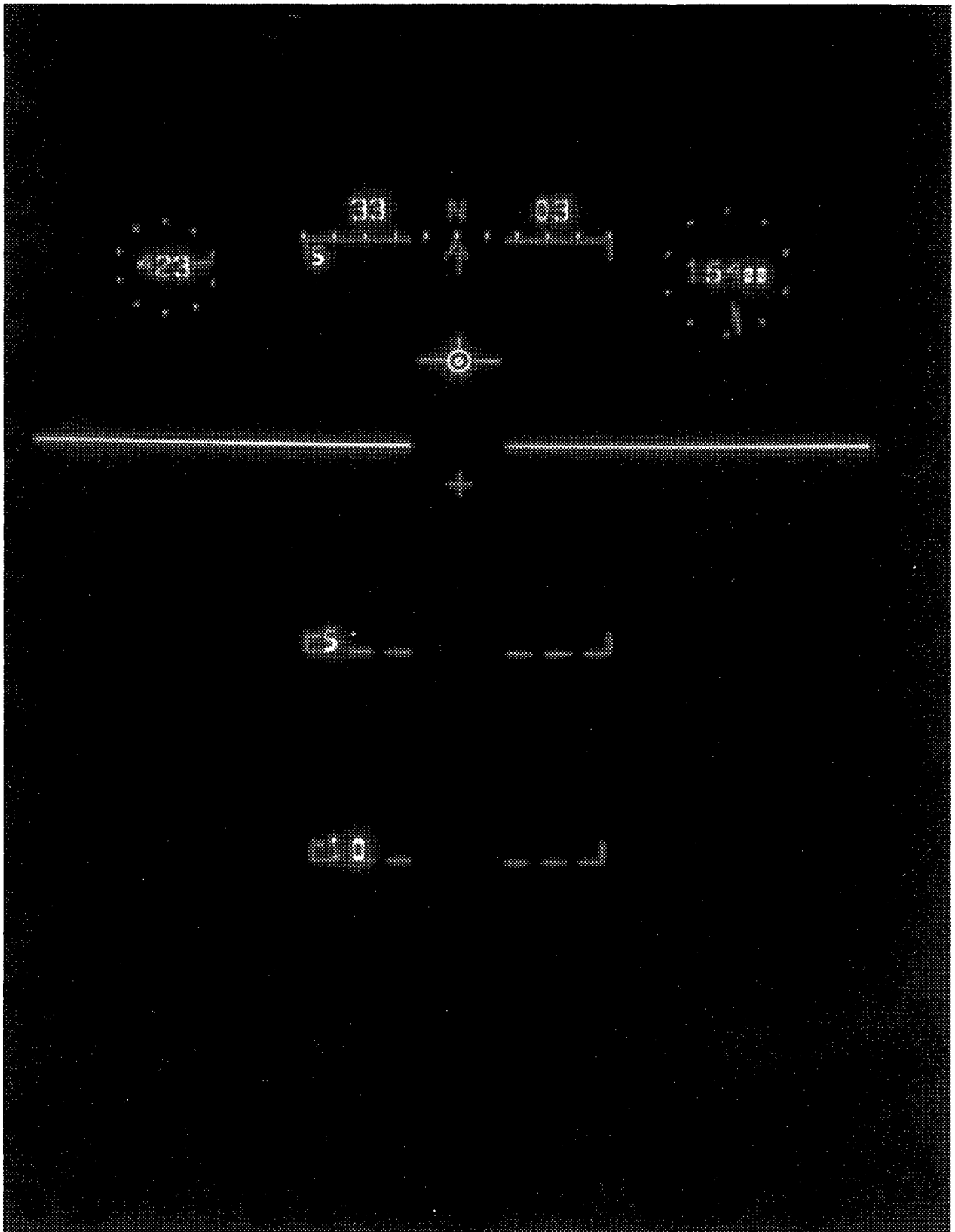
Figure 7. Basic HUD symbology.
