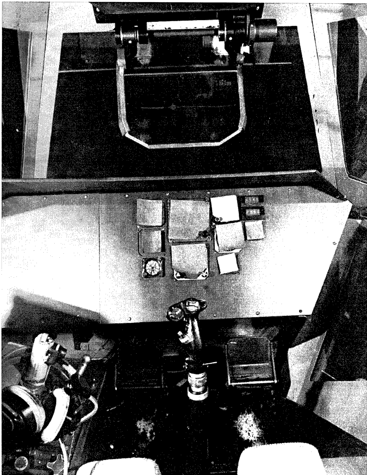
Figure 4. View of HUD and instrument panel (AC90-0178-67).
