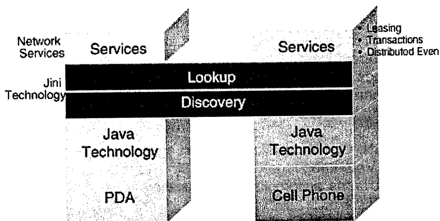
Figure 9: Jini Stack
