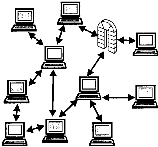
Figure 7: Distributed Arch
