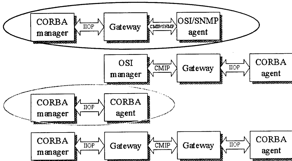
Figure 8 – JIDM Scenarios
