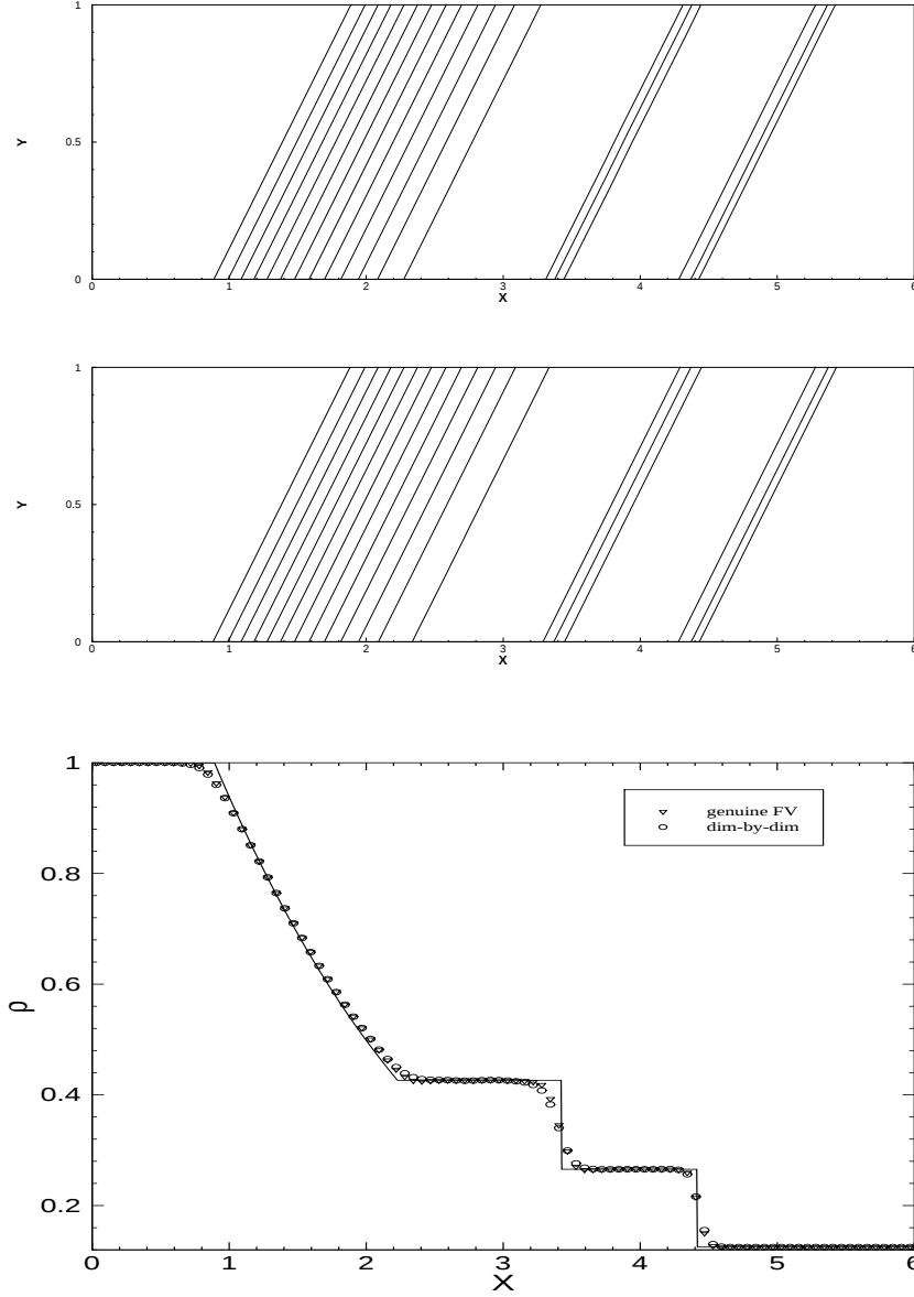
FIG. 3.1. Oblique Sod's problem. Density p . Top: contour, genuine two dimensional WENO; middle: contour, dimension by dimension WENO; bottom: cut at the bottom of the computational domain, the solid line is the exact solution, the triangles are the genuine two dimensional WENO results, and the circles are the dimension by dimension WENO results.
