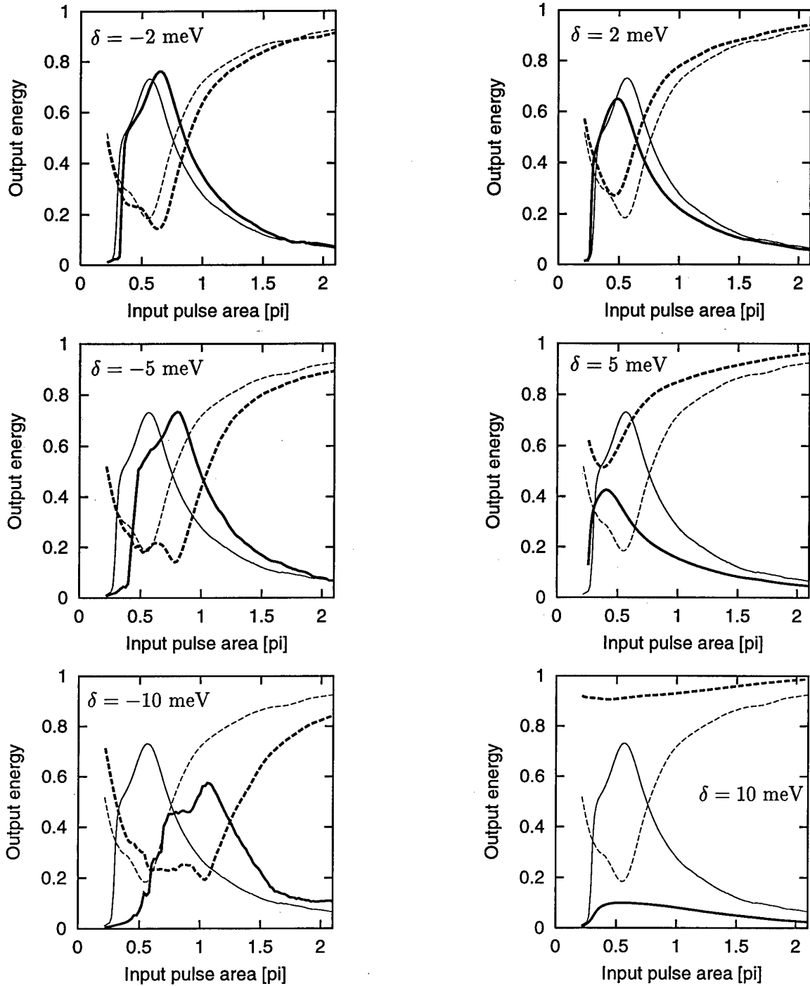
FIG. 2. Output energy (normalized to the input energy) vs. input pulse area for six different values of detuning of the pulse carrier frequency from the 1s -exciton resonance ( z = L_c ). An input 100-fs pulse is launched in channel 1 of the NLDC. Thick solid line shows an output of the NLDC in channel 1, and thick dashed line shows an output of the NLDC in channel 2. For comparison, thin solid and dashed lines show outputs in channels 1 and 2, respectively, in the case of on-resonance excitation ( \delta = 0 ). The switch response in the case of negative detunings (excitation above the resonance) and positive detunings (excitation below the resonance) is compared (see left and right columns, respectively).
