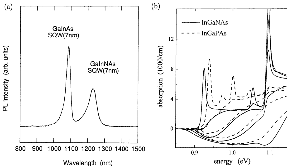
FIG. 7. (a) Photoluminescence spectra of InGaNAs and InGaAs at room temperature (the experimental results are taken from Ref. [19]). (b) Optical absorption and gain spectra for a 6 \text{ nm } \text{In}_{0.3}\text{Ga}_{0.7}\text{N}_{0.02}\text{As}_{0.98} QW between 10 \text{ nm} GaAs barriers (solid lines) and a 6 \text{ nm } \text{In}_{0.67}\text{Ga}_{0.33}\text{P}_{0.28}\text{As}_{0.72} QW between InP barriers (dashed lines) for carrier density (from top to bottom) of 0.25, 1.0, 2.5, 5.0 and 10 \times 10^{12} \text{ cm}^{-2} (the numerical results are taken from Ref. [22]).
