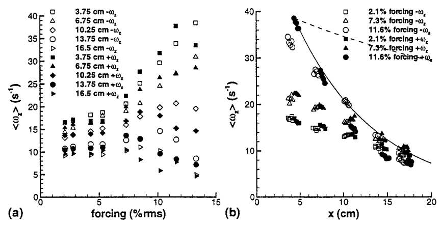
Figure 4: (a) Effect of forcing on peak vorticity magnitude at several downstream locations. (b) Variation of vorticity magnitude for 3 forcing amplitudes with respect to streamwise location. The solid line indicates the decay expected in the 11.6% forcing case solely due to negative stretching while the dashed line indicates the decay solely due to viscous diffusion.
