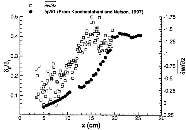
Figure 5: Comparison of mean \partial w/\partial z in 11.6% forcing case and \delta p/\delta_1 from Koochesfahani and Nelson (1997).
