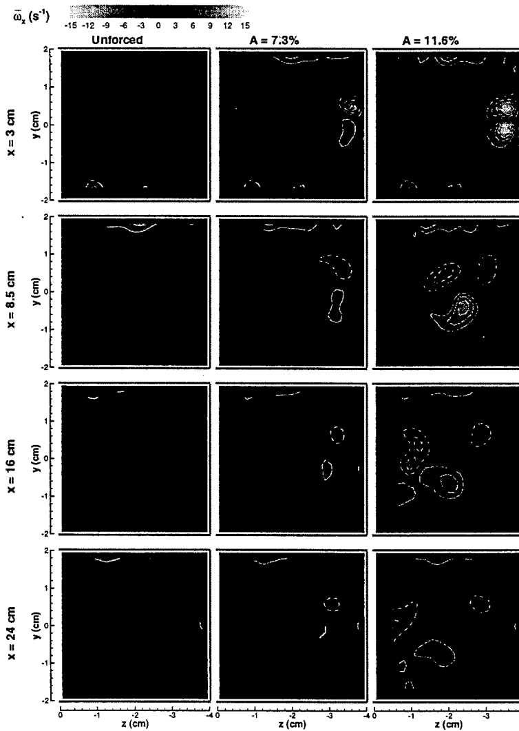
Figure 6: Mean streamwise vorticity field for the unforced, 7.3%, and 11.6% forcing cases at four downstream locations. Contour lines are spaced at \pm 3 \text{ s}^{-1} , \pm 6 \text{ s}^{-1} , ..., \pm 15 \text{ s}^{-1} . Dashed lines indicate negative vorticity.
