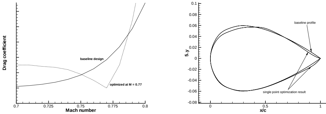
FIG. 2.1. Single point optimization: (a) drag profile and (b) geometry
