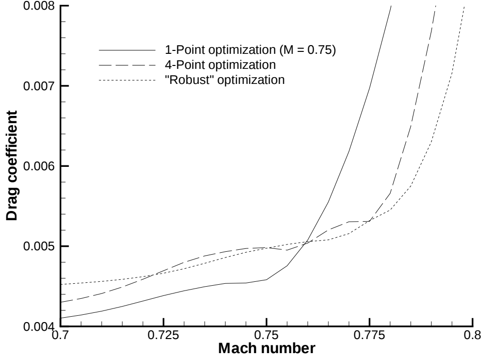
FIG. 4.1. Drag profile obtained using different optimization strategies
