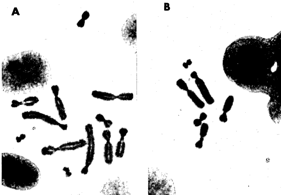
Figure 89. Colcemid-Metaphase Chromosome Spreads from the Rat Kangaroo Corneal Endothelium Cell Culture. (A) Cell with the normal diploid chromosome complement; (B) cell with a haploid chromosome complement.
