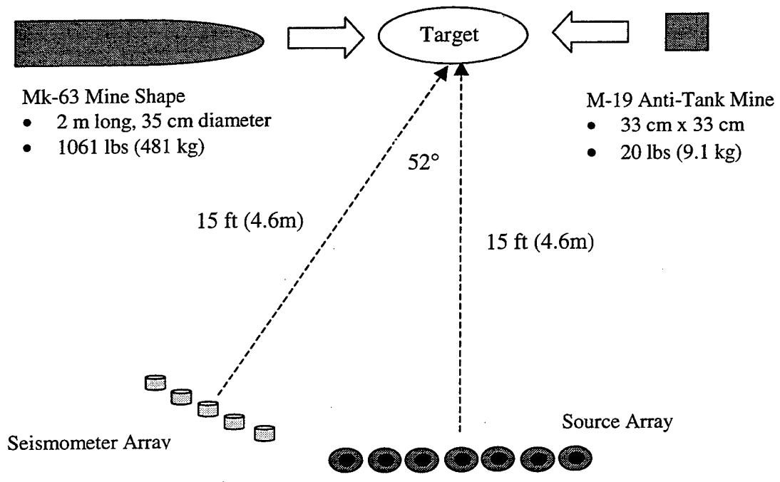
Figure 6.2. Bi-Static configuration used for detection experiments for Mk-63 mine shape and M-19 anti-tank mine.
