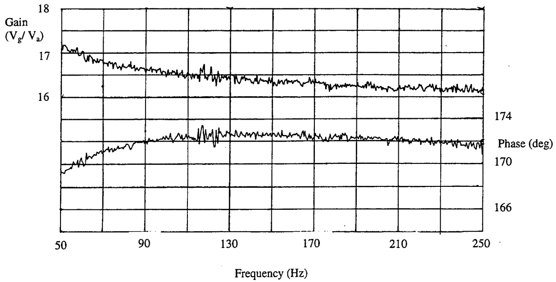
Figure 4.8. Phase relation and amplitude ratio between horizontal SM-6 geophone at zero degree tilt and a Bruel & Kjaer Type 8305S calibration accelerometer.
