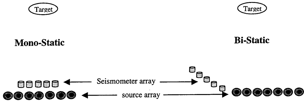
Figure 6.1. General mono-static and bi-static array configurations.
