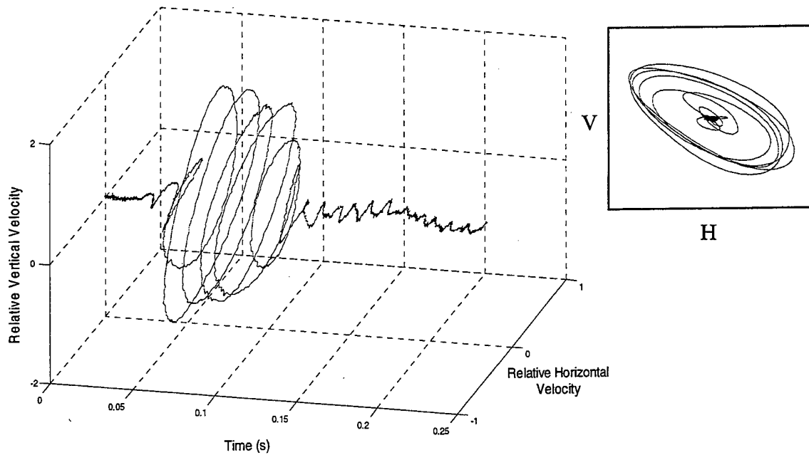
Figure 4.18. . Hankel plot of seismometer velocity signals measured 10 feet (3 m) from array of buried Bass Shaker paddles. Top right plot is the 2-D hodogram (V: vertical, H: horizontal).
