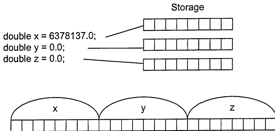
Figure 13.1.5.1a: Concatenating three doubles
