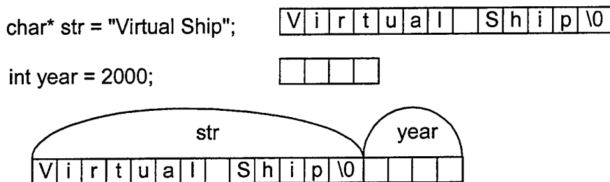
Figure 13.1.5.1b: Concetenating a string and an integer
