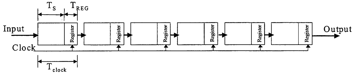
Figure 3. Pipelined Synchronous Process
