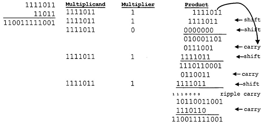
Figure 20. Carry-Save Addition Model
