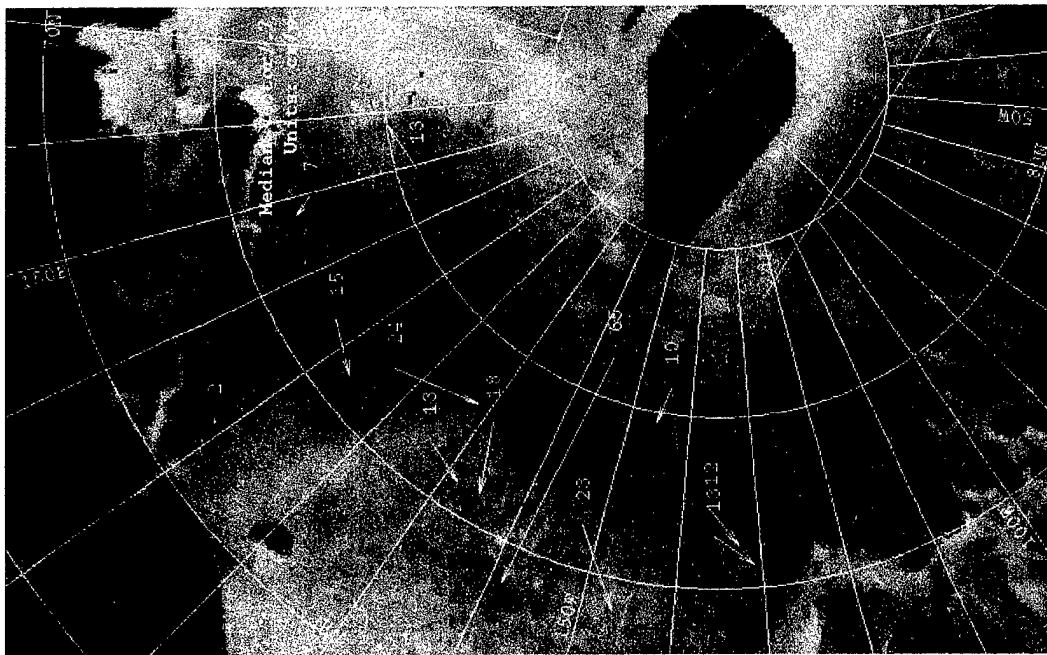
Figure 15. Median SSM/I motion vector match using a 0.7 and 0.9 correlation for December 29 th , 1999 at 1200Z.
