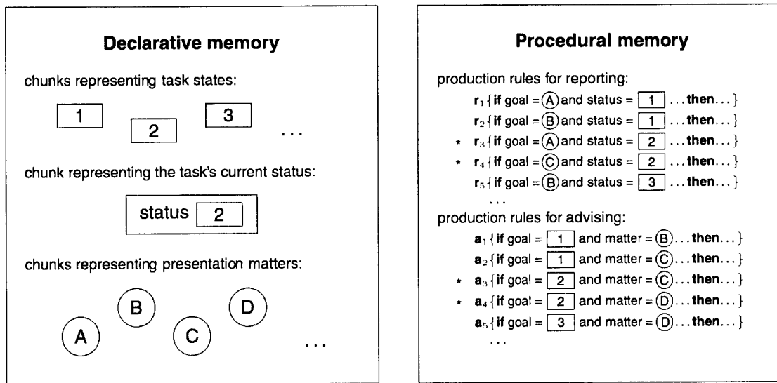
Fig. 7 — Anchoring production rules to presentation matters and the current status of the task. In addition to task states and the current status of the task (see Fig. 6, p. 29), matters that may warrant presentations—conceptual elements of the user's view of the task—are represented as chunks in the task model's declarative memory. The task model's display-based presentation functions (reporting and advising) are made up of many production rules (designated r_i and a_i in procedural memory in this illustration). Each rule is anchored the subject of its presentation and/or when it should be presented by specifying the corresponding presentation matter and task status chunks as a part of its condition for firing (i.e., in its if clause). Note that when a matter or the task's status is used as the task model's goal is a function of how the task model tracing system implements the presentation process (see material on the task model's presentation functions at p. 34 et seq. in Section 3.4.5). Depending on the goal (not shown in this illustration), the productions marked with an asterisk are those that are currently applicable to the state of the task model's declarative memory as it is depicted here.
