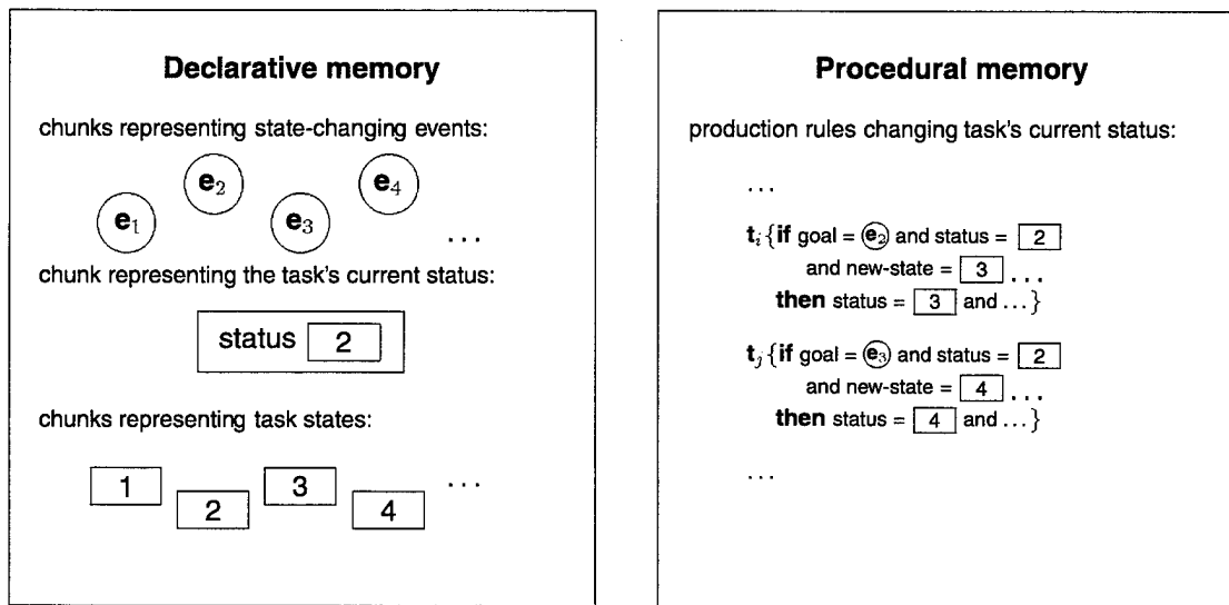
Fig. 6 — Representing task states and the task's current status in the task model. State-changing events and task states are represented as chunks in the task model's declarative memory. An additional chunk representing the current status of the task references the appropriate task state chunk in one of its slots. When a state-changing event occurs in the application, the chunk corresponding to it in the task model is made the goal. A specific set of production rules (designated t_i and t_j in this illustration) then carry out the appropriate transition. (The actual process is more elaborate than this simplified version indicates.) These actions are staged by the model as part of its addressee function. The task states shown in this illustration correspond to the notion of task junctures described later in this section on page 30 et seq.
