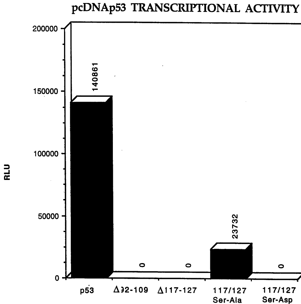
FIGURE 1 Transcriptional activity of pcDNAp53 constructs measured using a luciferase reporter plasmid in transfected Saos-2 cells.
