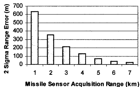
Figure 5.2-7 Moving Target Range Error versus Seeker Acquisition Range EO Handover.
