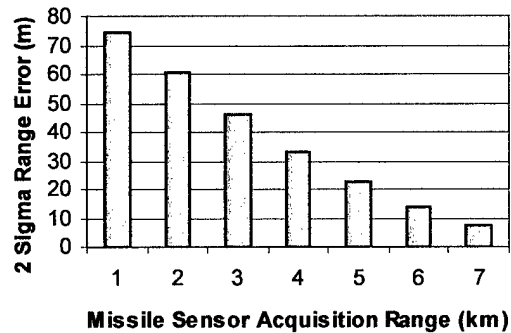
Figure 5.2-1 8k Stationary Target Range Error versus Seeker Acquisition Range RF Handover.
