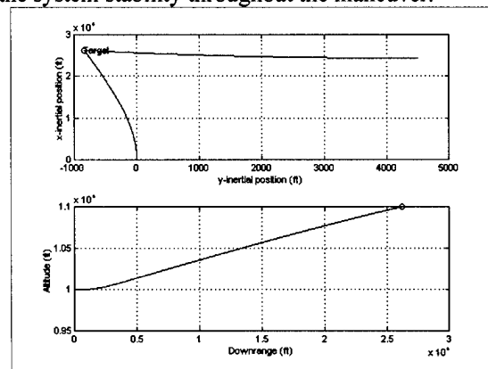
Figure 13. Missile and Target Position Time Histories
