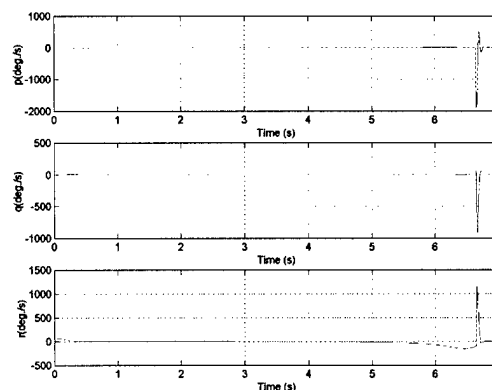
Figure 11. Roll, Pitch and Yaw Body Rate Histories
