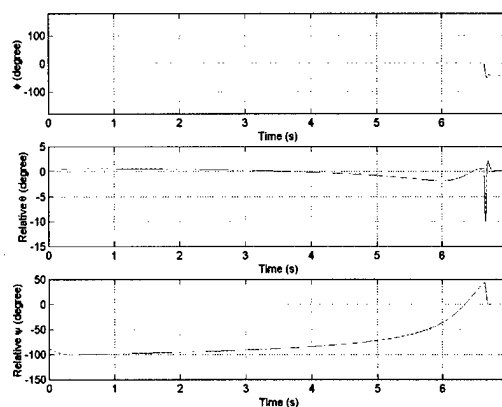
Figure 10. Roll, Pitch and Yaw Attitude Histories.
