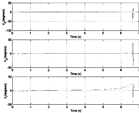
Figure 12. Roll, Pitch and Yaw Fin Deflection Histories
