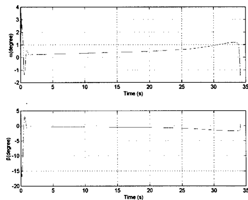
Figure 4. Angle-of-attack and Angle of Sideslip Time Histories
