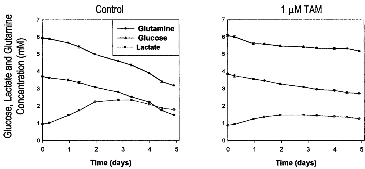
Figure 5: Glucose, lactate, and glutamine concentrations as a function of time for MCF7 microcarrier cultures.
