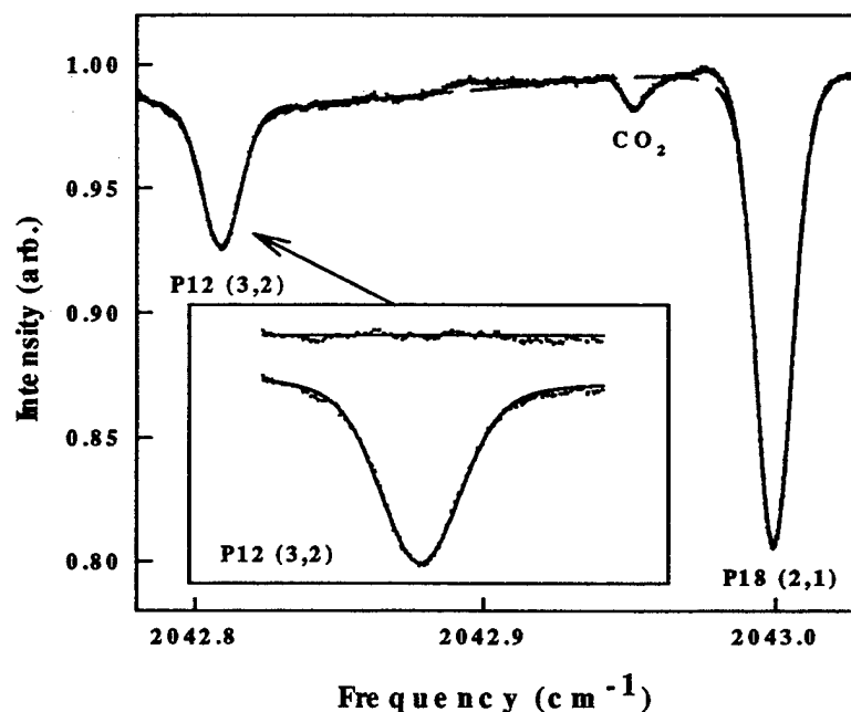
Figure 10. A Transmission Spectrum Measured Through a Low-Pressure, Premixed CH 4 /O 2 Flame at 20 Torr. The Main Absorption Features Are the Two CO Lines Used to Calculate the Temperature Using the Method of Two-Line Thermometry. Calculated Temperature Was 2,150 K.
