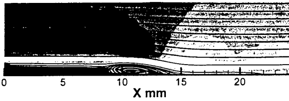
c) 25.4% of input waveform, flap deflection = 22.3 \mu m
