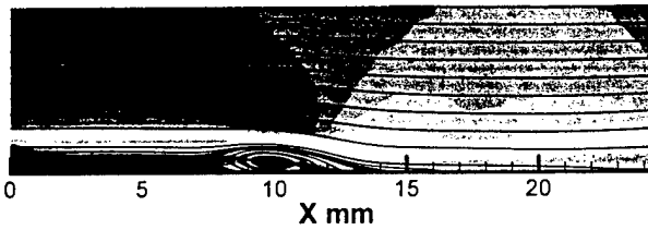
b) 15.4% of input waveform, flap deflection = 22.5 \mu m
