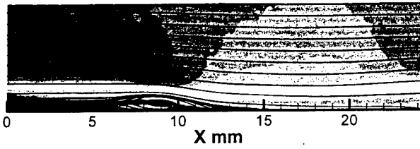
a) 5.4% of input waveform, flap deflection = 14.1 \mu m
