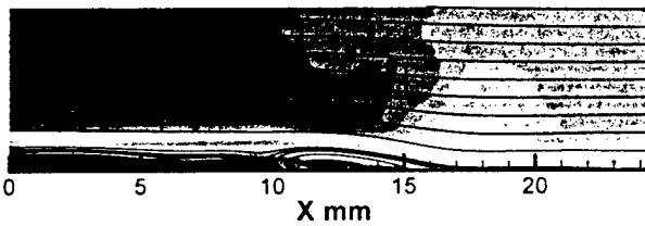
d) 35.4% of input waveform, flap deflection = 13.6 \mu m
