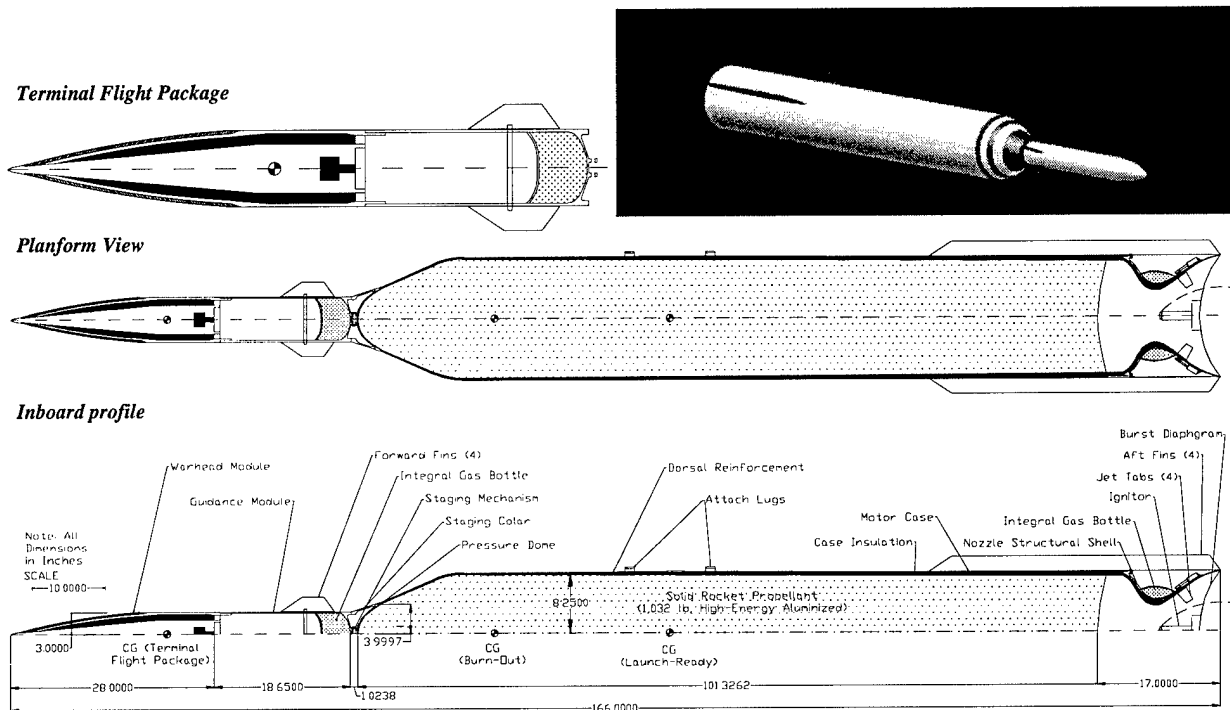
Figure 2: DKM119-7R Configuration, Inboard Profile, and Major Design Details.
