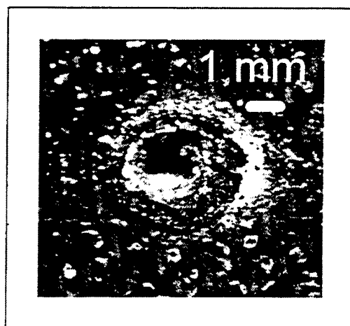
Figure 43. Polyimide hole 5. Intensity 10 \text{ kW/cm}^2 , with air. Average Power 100 W. Spot Radius 0.87 mm.
