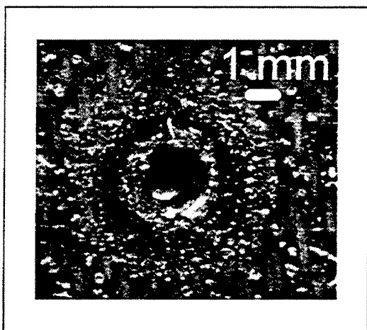
Figure 42. Polyimide hole 8. Intensity 10 \text{ kW/cm}^2 , no air. Average Power 100 W. Spot Radius 0.87 mm.
