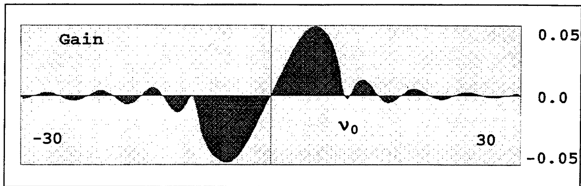
Figure 8. FEL Gain Spectrum, j=2 , \alpha_0 = 20 .
