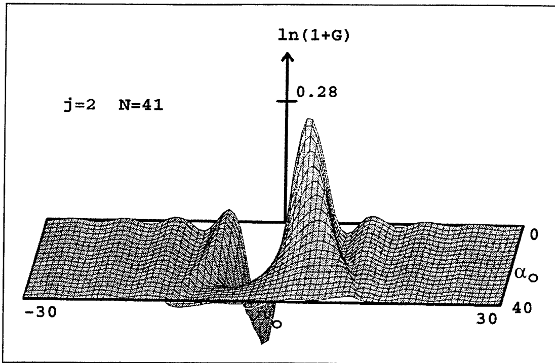
Figure 6. FEL Gain Spectrum, j=2 .
