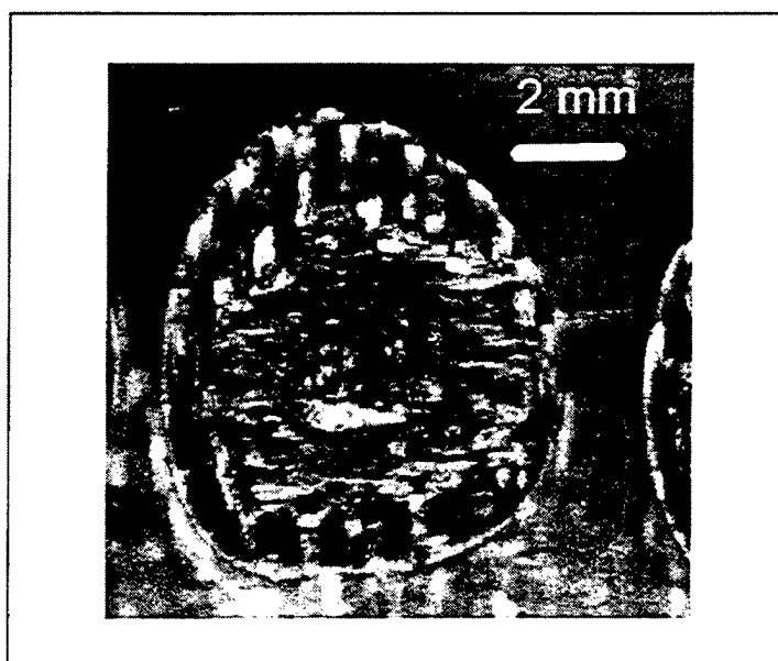
Figure 52. Epoxy, hole 5. Intensity 500 \text{ W/cm}^2 , with airflow. Average Power 100 W. Spot Radius 2.5 mm.
