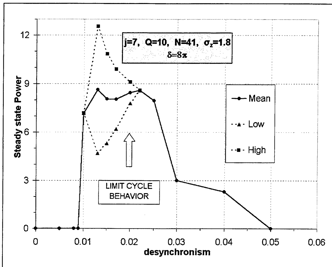
Figure 35. Desynchronism Curve for \delta=8\pi .
