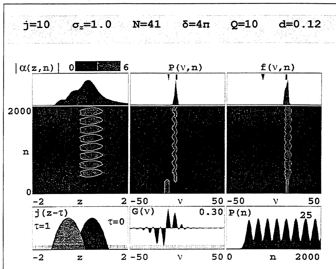
Figure 26. Limit-cycle behavior.
