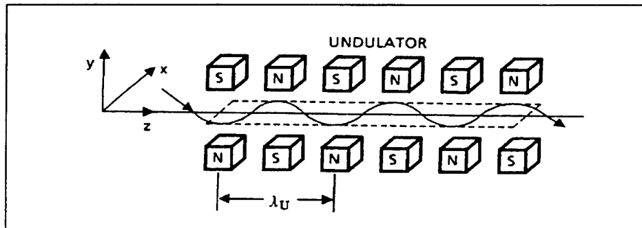
Figure 4. Electron motion inside the Undulator. (From Ref. 2).
