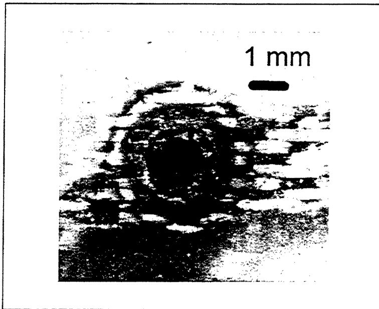
Figure 55. Epoxy, hole 12. Intensity 10 \text{ kW/cm}^2 , no air. Average Power 100 W. Spot Radius 0.87 mm.
