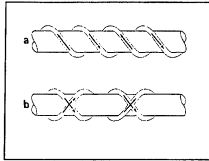
Figure 3. Linear Undulator. (From Ref. 2).
