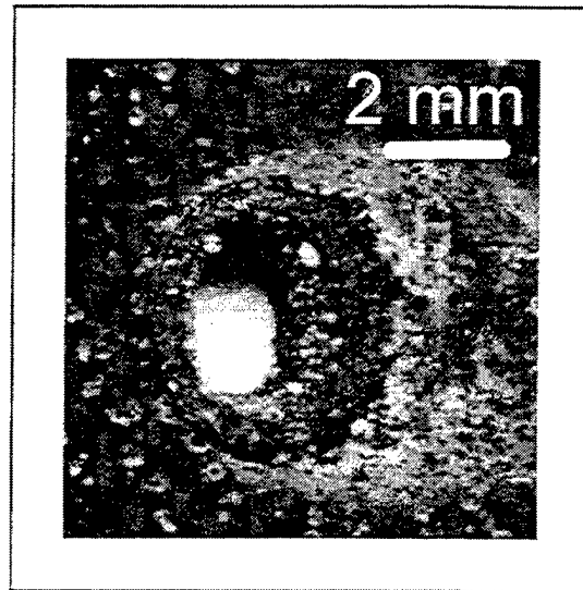
Figure 45. Polyimide hole 20. Intensity 10 \text{ kW / cm}^2 , with air. Average Power 500 W. Spot Radius 1.25 mm.
