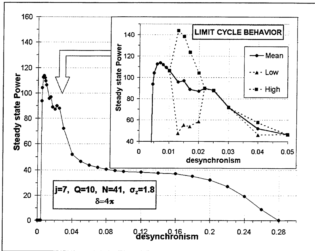
Figure 34. Desynchronism Curve for \delta=4\pi .
