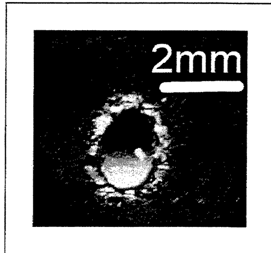
Figure 47. Polyimide exit hole 20. Intensity 10 \text{ kW / cm}^2 , with air. Average Power 500 W. Spot Radius 1.25 mm.
