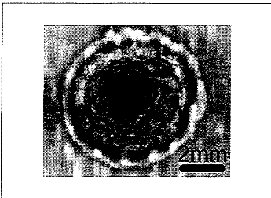
Figure 53. Epoxy, hole 16. Intensity 10 \text{ kW/cm}^2 , no air. Average Power 500 W. Spot Radius 1.25 mm.
