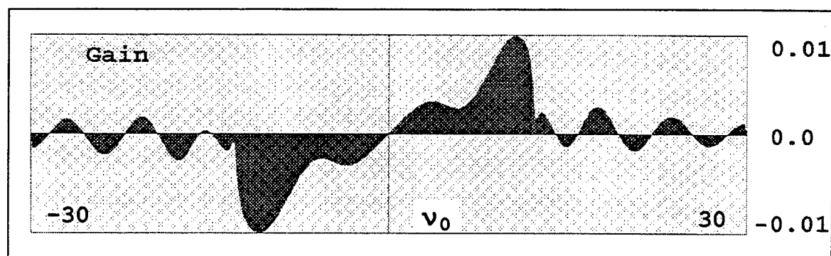
Figure 9. FEL Gain Spectrum, j=2 , \alpha_0 = 40 .
