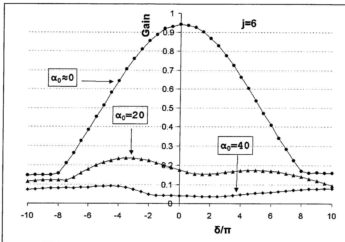
Figure 20. Plot of peak gain versus tapering rate.
