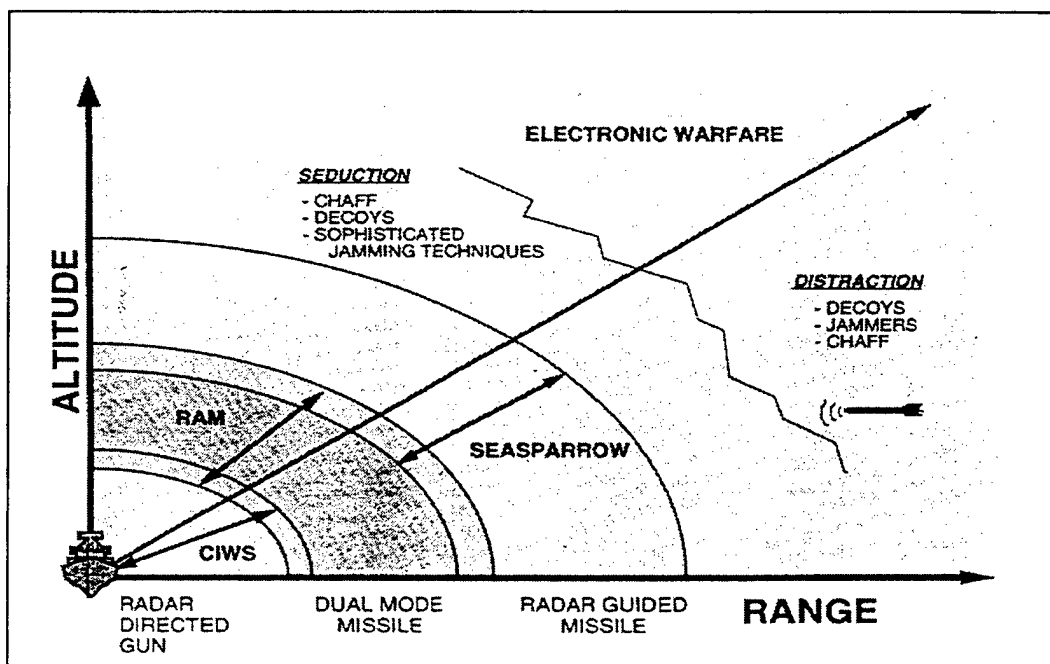
Figure 10. Layered Ship Self-defense. (From Ref. 10).
