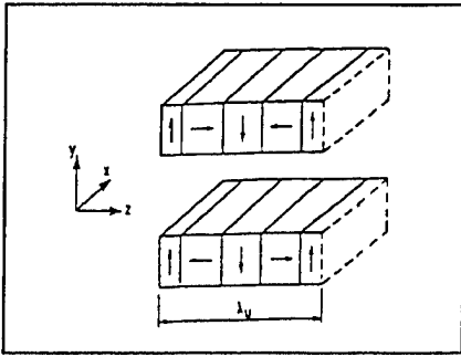
Figure 2. Helical Undulator. (From Ref. 2).
