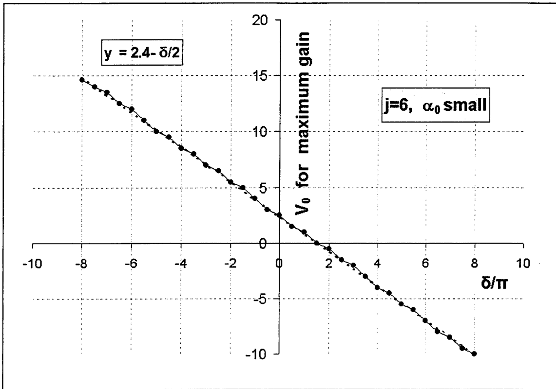
Figure 21. Position of Peak Gain versus taper.
