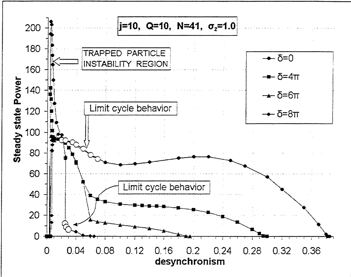
Figure 25. Desynchronism Curve for various tapering rates.
