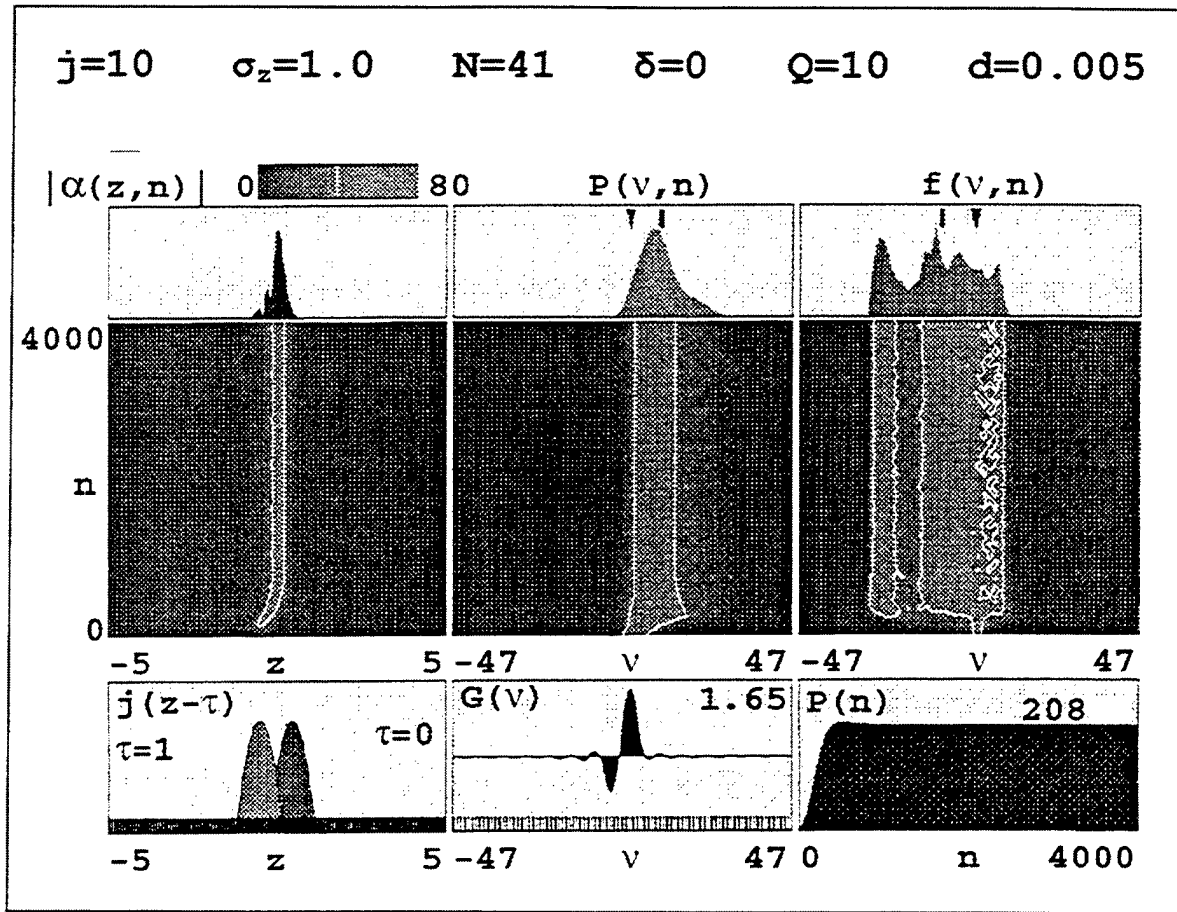
Figure 24. Trapped Particle Instability.
