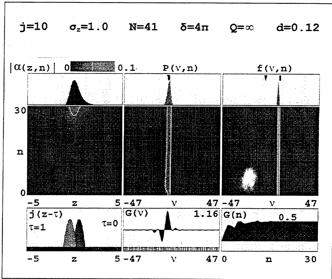
Figure 27. FEL Short Pulse and Gain Evolution.
