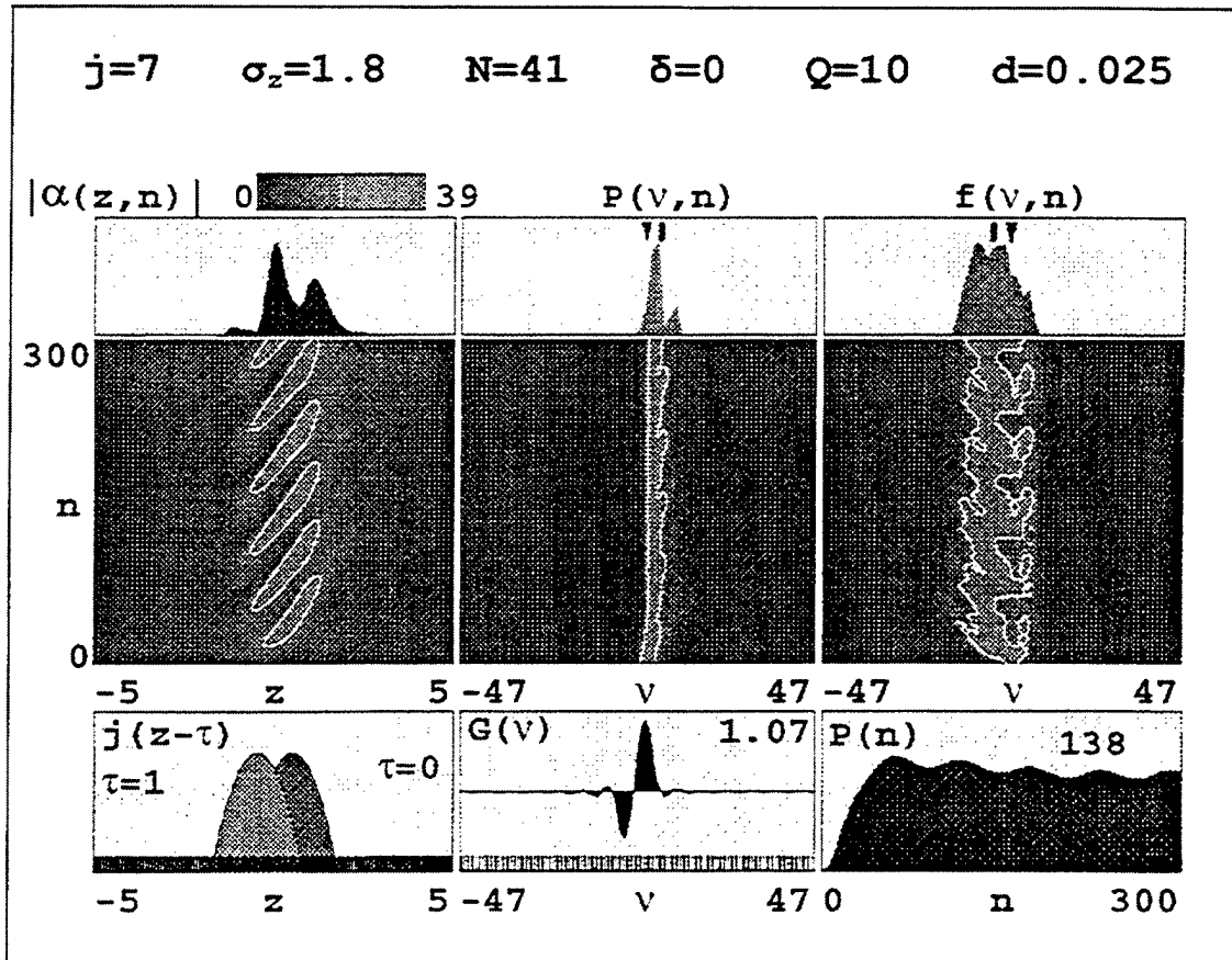
Figure 32. Simulation Output for d=0.025 and \delta=0 .
