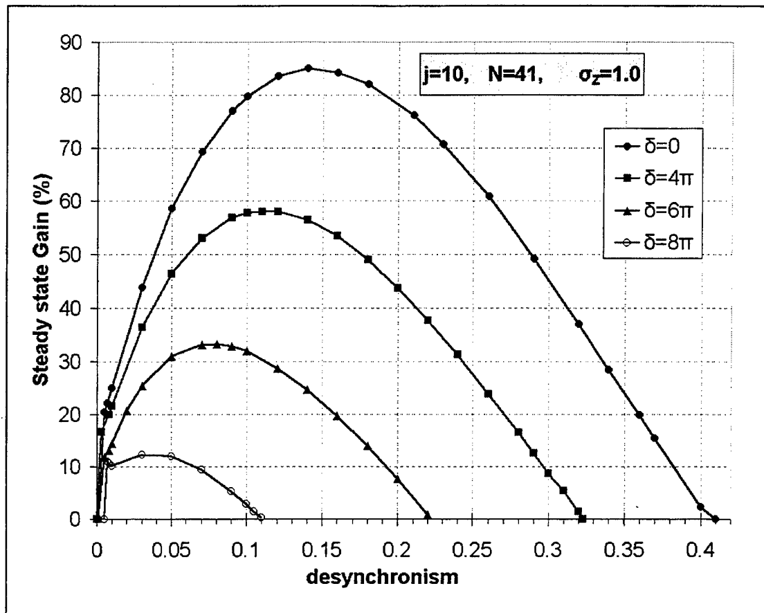
Figure 28. Steady State Gain versus desynchronism
