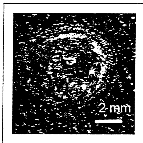
Figure 41. Polyimide hole 15. Intensity 500 \text{ W/cm}^2 with air. Average Power 100 W. Spot Radius 2.5 mm.
