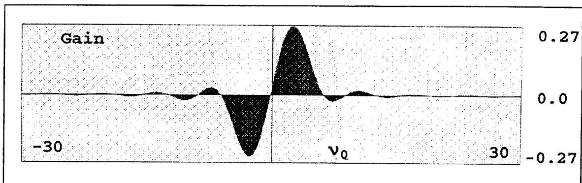
Figure 7. FEL Gain Spectrum, j=2 , \alpha_0 = 0 .
