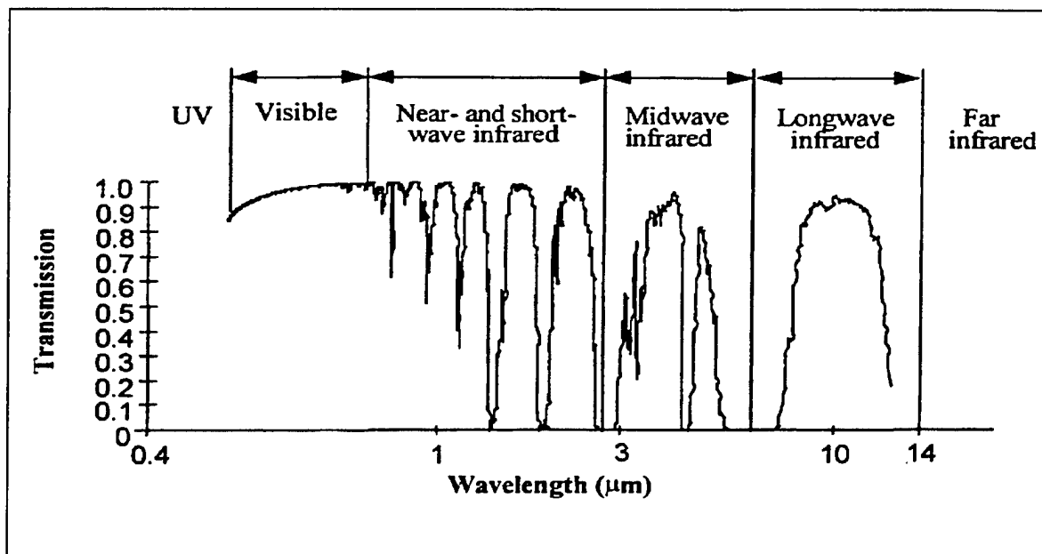
Figure 15. Atmospheric Transmittance. (From Ref. 5).
