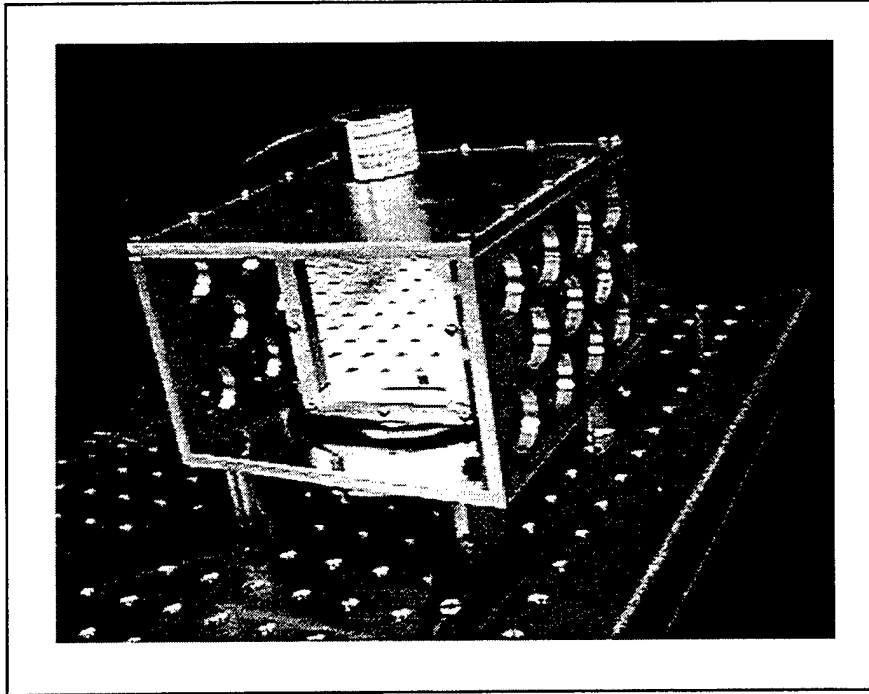
Figure 3.8. The mirror optomechanical scanner, consisting of supporting cage, servo motor, rotary encoder, mirror housing and mirror.
