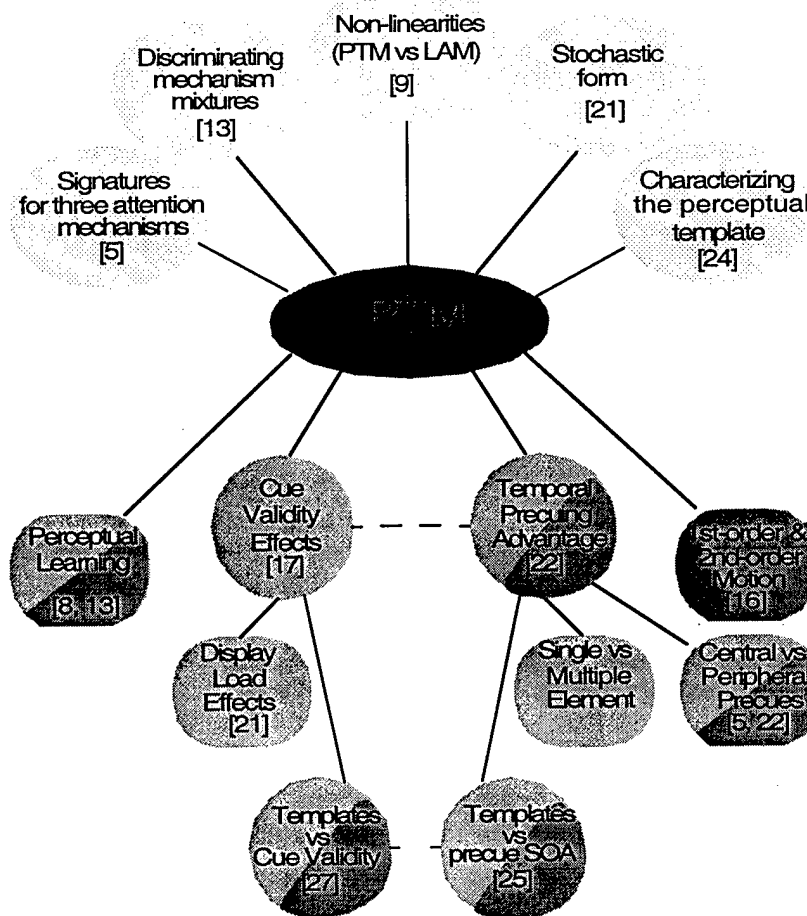
Figure 1. A roadmap of work from the prior grant period. Theoretical findings (top) and empirical findings of external noise exclusion (light gray) and stimulus enhancement (dark gray) (bottom).
