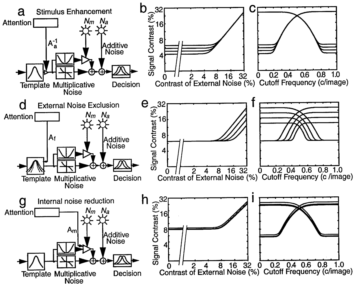
Figure 2. Three mechanisms of visual attention and their performance signatures. (b,e,h) show attention effects on threshold contrasts with increasing external noise levels; (c,f,i) show attention effects on threshold contrasts for filtered external noise as a function of cutoff frequency.
