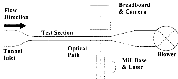
Figure 6 - Overall Setup
