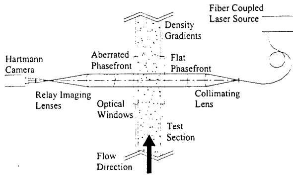
Figure 7 – Optical Arrangement
