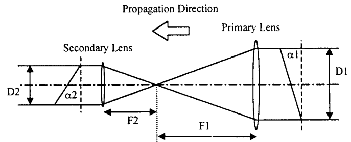
Figure 3 – Relay-Imaging Optics
