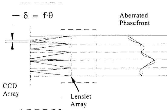
Figure 2 – Displacement of Focal Spot
