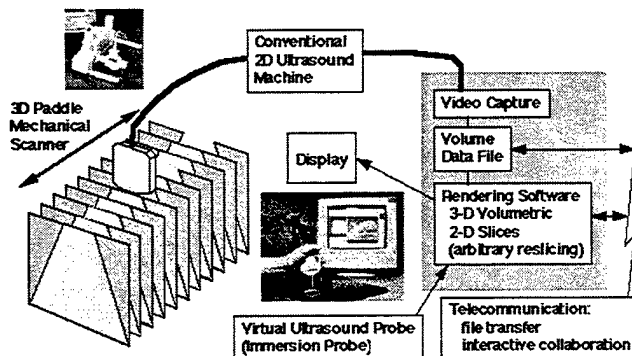
Figure 6. Major components, operations, and data flows in MUSTPAC-1.
