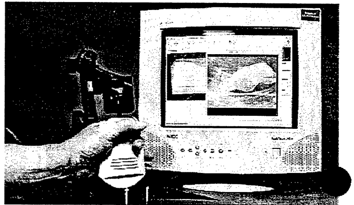
Figure 3. Closeup of the Virtual Ultrasound Probe and diagnostic workstation display.
