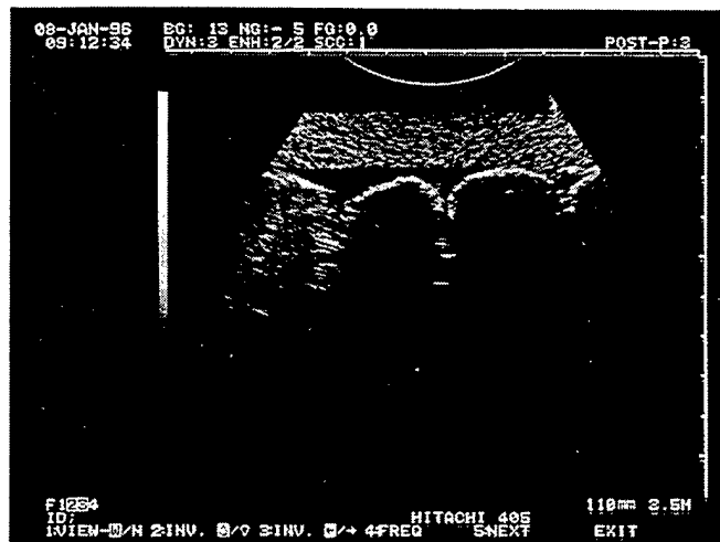
Figure 4. B-Scan Image of Blood Pool Phantom (3.5 MHz)
