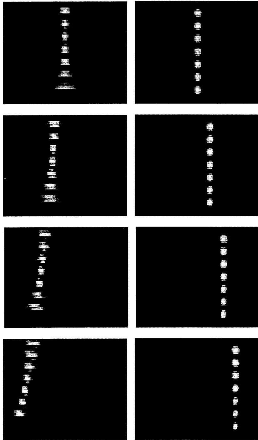
Figure 13 Comparison of time-domain waveform images (left) and full wideband reconstructed images (right) for seven point scatterers at depths ranging from 1.3 to 1.9 times the aperture width at various positions across the aperture.
