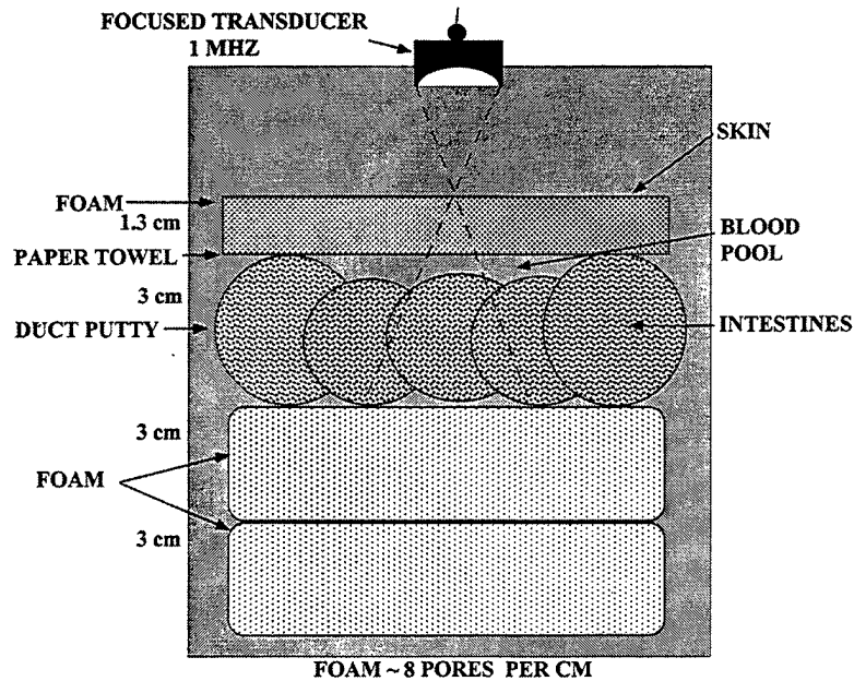
Figure 7. Blood Pool Phantom in water tank for 1 MHz Imaging Tests
