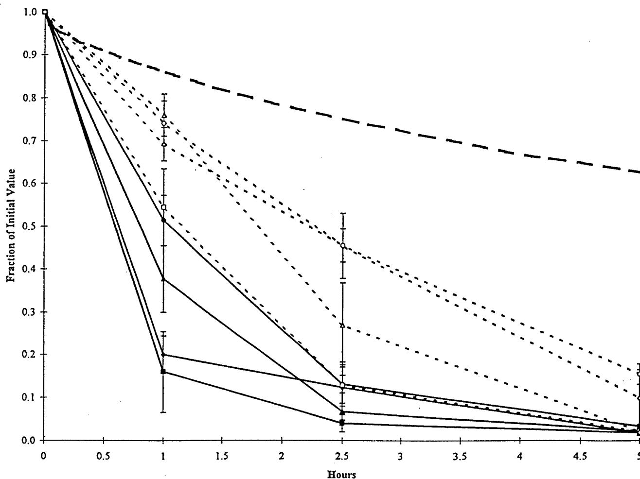
Figure 1. Evaporation of naphthalene from Jet-A (—◆—), JP-8 (—■—), JP-8(100) (—▲—), and JP-8(Puddle) (—●—) jet fuels, and evaporation of total JP-8 (---) jet fuels, and evaporation of naphthalene from Jet-A (---◆---), JP-8 (---□---), JP-8(100) (---△---), and JP-8(Puddle) (---○---) jet fuels.
