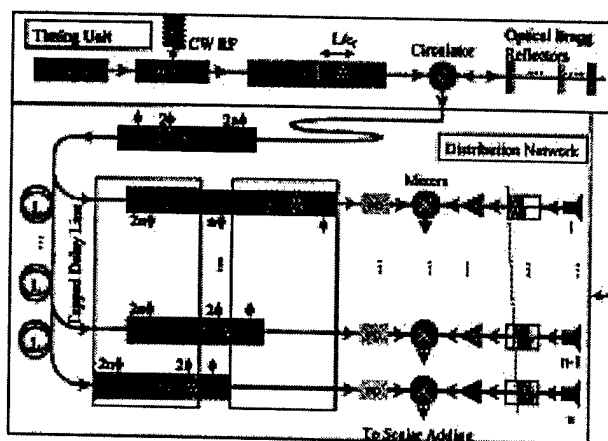
Fig. 1. Basic serially fed receive mode configuration for an array of n elements. A chirped fiber grating in conjunction with a tunable laser provides the necessary phased delays for virtually continuous directional operation. A second tapped delay line in parallel can be added to achieve almost continuous temporal operation.
